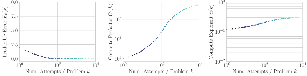
Figure 4: Pretraining Compute Scaling Law Parameters by Number of Attempts per Problem (Full Fits). We visualize how the parameters of Eqn. 3 change with respect to k . Hue corresponds to k .
