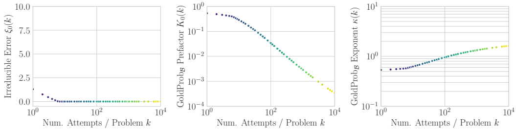
Figure 6: Gold Reference Log Likelihoods Scaling Law Parameters by Number of Attempts per Problem (Full Fits). We visualize how the parameters of Eqn. 5 change with respect to k . Hue corresponds to k .
