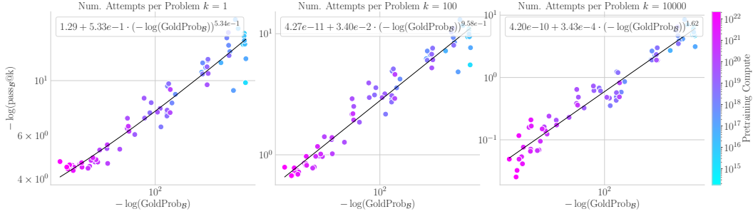
Figure 11: Scaling of Pass Rates with Gold Reference Likelihood (Full Fit). Each panel fits Eqn. 6, -\log(\text{pass}_B@k) = \xi_0 + K_0(k) \cdot [-\log(\text{GoldProb}_B)]^{\kappa(k)} , for k \in \{1, 10^2, 10^4\} . Regressing the gold reference log-likelihoods against the pass rates produces a visually tighter fit with less residual scatter than the compute scaling law (cf. Fig. 1). As k increases, the irreducible error \hat{\xi}_0(k) falls toward zero and the exponent \hat{\kappa}(k) increases, making the relationship a steeper, purer power law.
