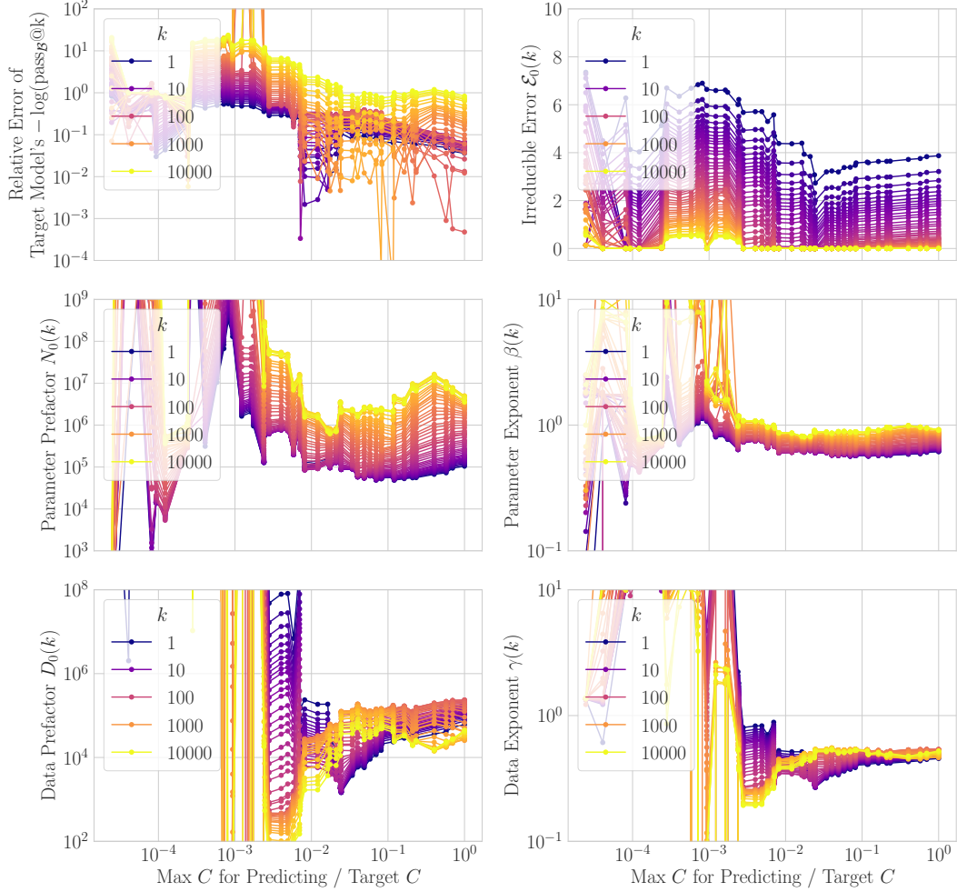
Figure 8: Predicting Pass Rates from Scaling Parameters and Tokens (Backtesting) . We evaluated how accurately the parameters + tokens scaling law (Eqn. 4) predicts the most expensive model’s -\log(\text{pass}_B@k) . Top Left: The relative error decreases as higher-compute checkpoints are included, plateauing once the fit includes models within \sim 2 orders of magnitude of the target. Other Five Panels: The estimates of the five scaling law parameters are initially unstable but converge to their full-fit values once included models are within \sim 2 orders of magnitude of the target.
