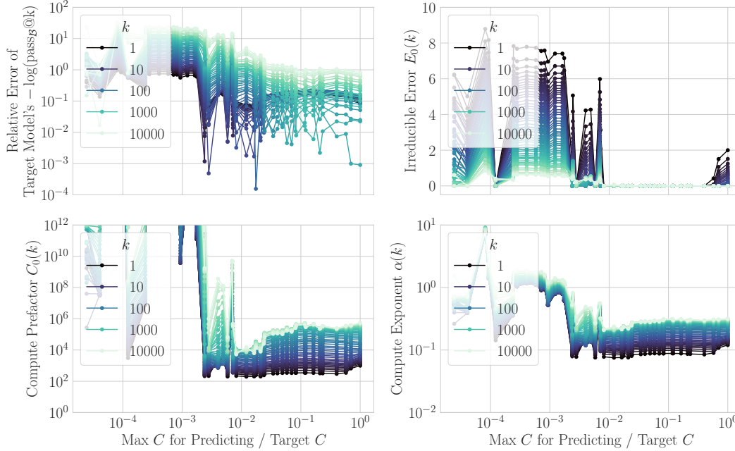
Figure 7: Predicting Pass Rates from Scaling Pretraining Compute (Backtesting). We evaluate predictability via backtesting : we iteratively fit Eq. 3 on subsets of models up to a maximum pretraining compute, then extrapolate to predict the most expensive model’s -\log(\text{pass}_B@k) . The most expensive model is Pythia 12B-parameter 300B-token ( \approx 2.16 \times 10^{22} FLOP). The x -axis in all panels is the ratio of the largest-compute checkpoint included in the fit to the target model’s compute. Top Left: Relative error decreases as higher-compute checkpoints are included and then plateaus: for k \in \{1, 10^2\} the plateau occurs once the fit includes checkpoints within \sim 2 orders of magnitude of the target; for k=10^4 it occurs within \sim 1.5 order. Other Three Panels: Backtested estimates of the scaling law parameters converge as the fit includes higher-compute checkpoints, stabilizing to full-fit values once included models are within \sim 2 orders of magnitude of the target.
