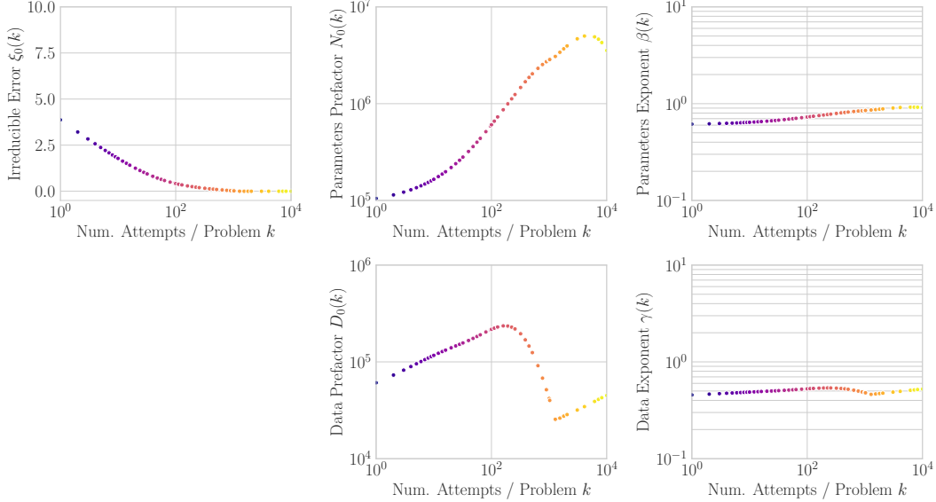
Figure 5: Model Parameters and Tokens Scaling Law Parameters by Number of Attempts per Problem (Full Fits). We visualize how the parameters of Eqn. 4 change with respect to k . Hue corresponds to k .
