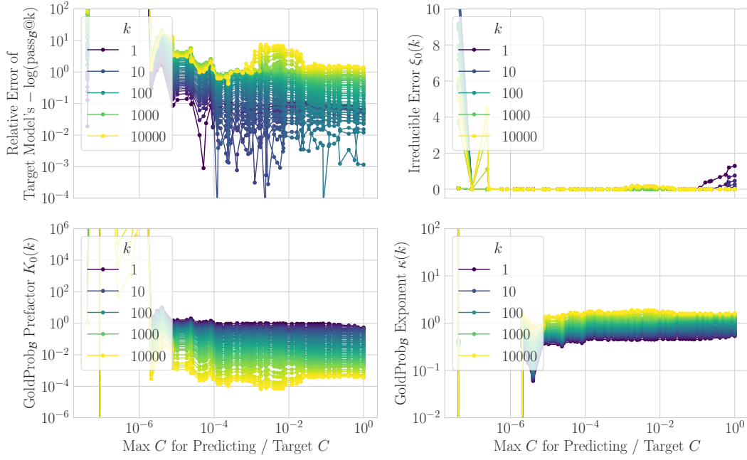
Figure 9: Predicting Pass Rates from Gold Reference Likelihoods (Backtesting). While the overall predictive error is comparable to the other laws, it is slightly lower for small k and slightly higher for large k . Top Left: The most striking result is the exceptional stability of the scaling law’s parameters. In stark contrast to the compute and parameters+tokens laws, whose parameters stabilized only when fit on models within \sim 2 orders of magnitude of the target, the backtested estimates for \hat{\xi}_0(k) , \hat{K}_0(k) , and \hat{\kappa}(k) converge to their final values using models up to \sim 5 orders of magnitude cheaper than the target. Other Three Panels: This remarkable stability suggests that the relationship between gold reference likelihoods and pass rates provides a robust signal, enabling reliable, long-range forecasts from much cheaper models.
