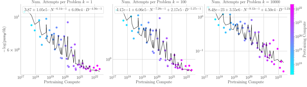
Figure 10: Scaling of Pass Rates with Model Parameters and Pretraining Data (Full Fit). Each panel fits Eqn. 4, -\log(\text{pass}_B@k)(N, D, k) = \mathcal{E}_0(k) + N_0(k) N^{-\beta(k)} + D_0(k) D^{-\gamma(k)} . Relative to the compute scaling law, using parameters N and tokens D instead yields tighter in-range fits for all k . Consistent with Fig. 2, the irreducible error decreases sharply with k (e.g., \hat{\mathcal{E}}_0: 3.87 \rightarrow 0 by k \approx 10^2 ), after which variation is dominated by the (N, D) terms. Despite the better global fit, the largest-compute model checkpoint in each panel exhibits comparatively large relative error.
