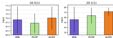
Figure 2: Comparison of average hIoU scores over three different category orderings on PASCAL VOC [10].
