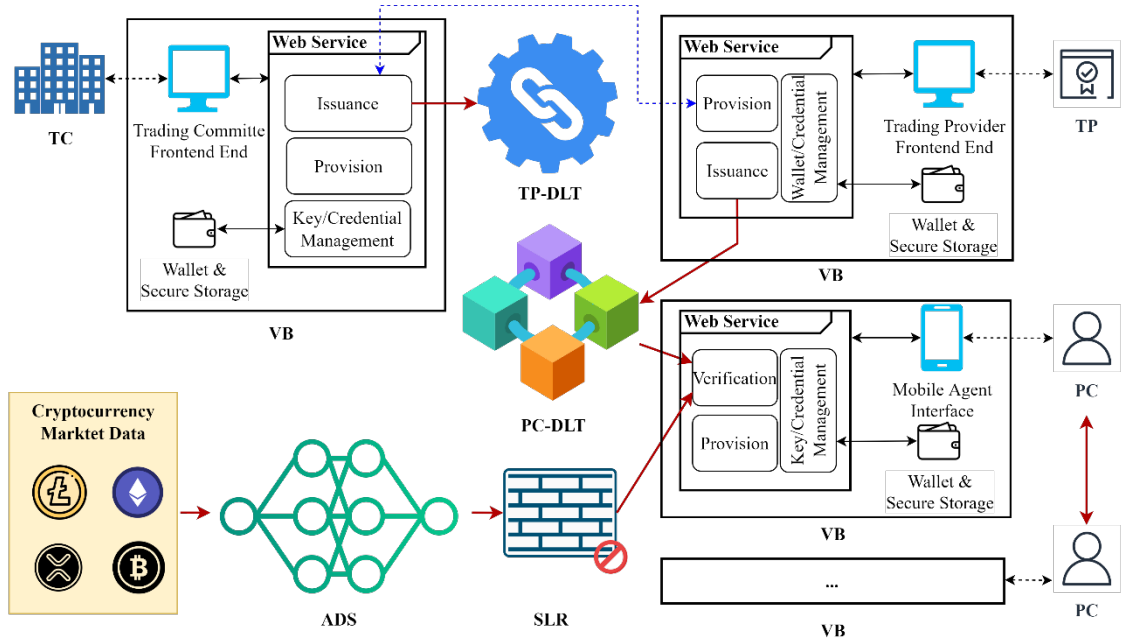
Figure 1. ADPP Architecture
