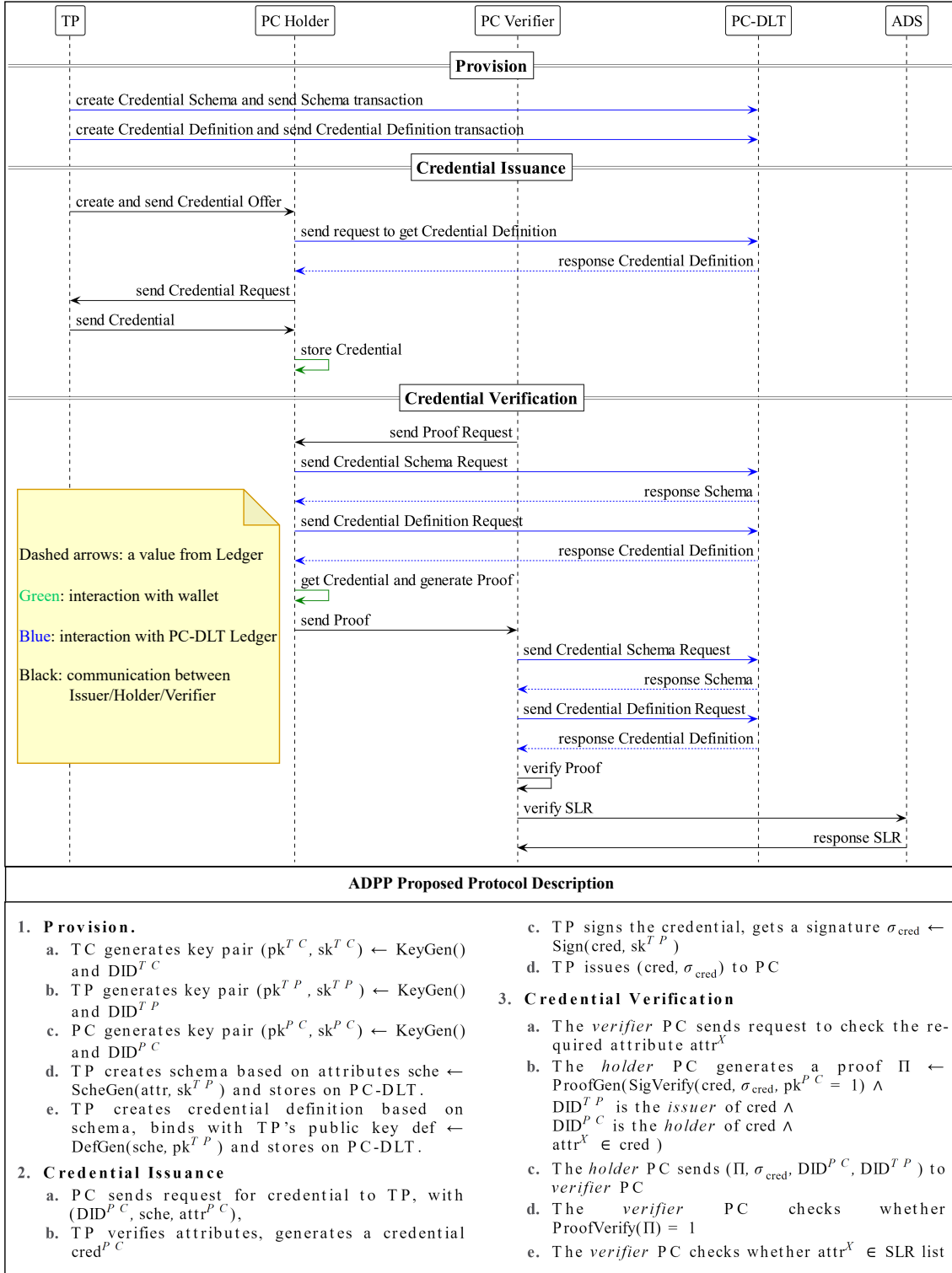
Figure 2. Protocol Description
