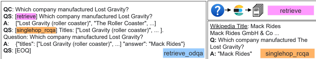
Figure 6: A Decomposed Prompt to answer open-domain questions using Elasticsearch-based retrieval. Full usage of this prompt for open-domain multihop questions is given in Fig. 11.
