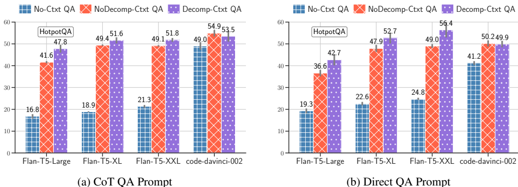
Figure 14: Results on HotpotQA dataset
