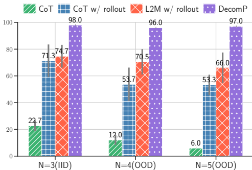
Figure 7: EM Results on the k^{th} letter concatenation task (k=3) using space as delimiter with different number of words in the input. DECOMP outperforms and generalizes better than CoT as well as Least-to-most prompting.
