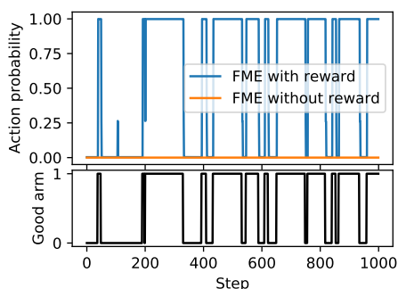
Figure 2. Given the reward as input, self-modifications enable adaptation to swapping of the good arm in a two-armed bandit.
