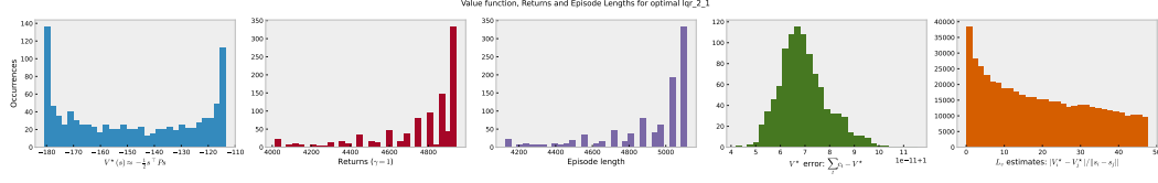
Figure 8: Statistics for 1qr_2_1. The right-most histogram justifies the choice of L \approx 50 .
