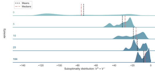
Figure 5: Distribution of the suboptimality gap V^\pi(s_0) - V^*(s_0), s_0 \sim \rho at different stages of training on lqr_2_1 . See the caption in Figure 4 for experiment details. The gap shrinks as training progresses, and at the last episode our algorithm certifies with high probability the desired gap of \varepsilon = 50 .
