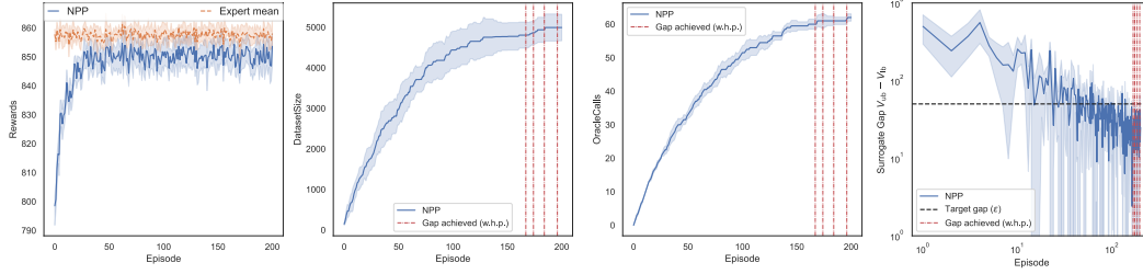
Figure 4: Training curves for lqr_2_1 with target suboptimality \varepsilon = 50 , with results averaged over 4 seeds. Left : Episodic return of policy \pi (in blue) and expert (in orange) at different stages of training. N = 100 rollouts are performed at each point; solid line corresponds to the median and shaded area to a 95% confidence interval. Middle-left : size of the dataset. Middle-right : calls to the TrajectoryOptimizer oracle (notice calls are made on approximately 30% of the episodes). Right : surrogate gap V_{ub} - V_{lb} for the initial states. Purple dashed lines correspond to the hitting times (one per seed) for reaching the target suboptimality gap.
