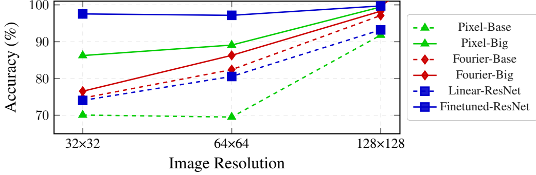
Figure 3: Classification accuracy comparison across different model architectures on the OrganAMNIST dataset. Results show performance scaling with image resolution from 32×32 to 128×128 pixels. Fine-tuned ResNet consistently achieves the highest accuracy across all resolutions.
