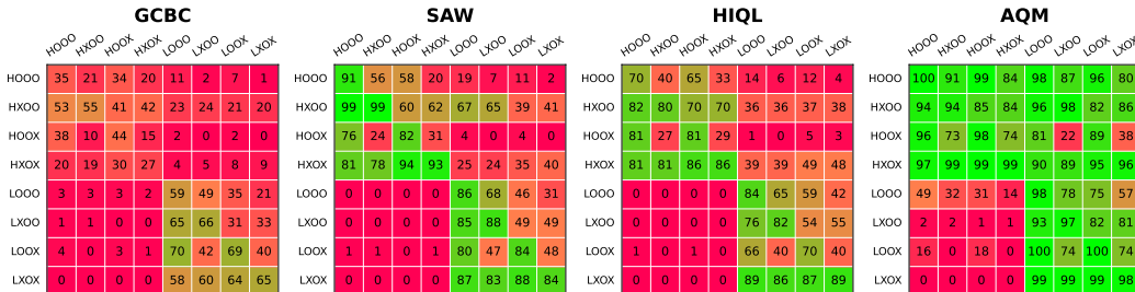
Figure 9: Evaluating Test-time Adaptation. Performances are presented as heatmaps where rows represent the training environment and columns represent the evaluation environment. The diagonal values represent standard evaluation setup (training and evaluation environments match), while off-diagonal entries quantify test-time replanning capabilities under specific environmental shifts.
