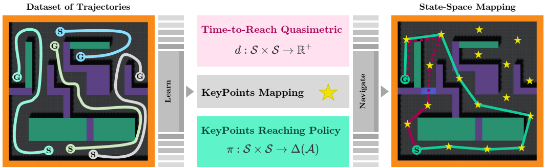
Figure 1: Adaptive Quasimetric Mapping (AQM) . (left) We leverage \mathcal{D} = \{\tau_i = (s_0^{(i)}, a_0^{(i)}, \dots, s_T^{(i)})\} a dataset of trajectories ; (middle) we learn a time-to-reach quasimetric d : \mathcal{S} \times \mathcal{S} \rightarrow \mathbb{R}^+ , a goal-conditioned policy \pi : \mathcal{S} \times \mathcal{S} \rightarrow \Delta(\mathcal{A}) ; (right) and the quasimetric is used to build a sparse topological graph of the state space, with keypoints (★) providing near uniform coverage of the dataset support. During inference, AQM plans a path from a starting position (S) to a goal (G) and follows it using the learned policy. It can adapt to topological changes at test-time, such as a blocked path , by monitoring budget overruns given predicted time-to-reach values. Consequently performing zero-shot replanning, to reach the goal through another feasible path .
