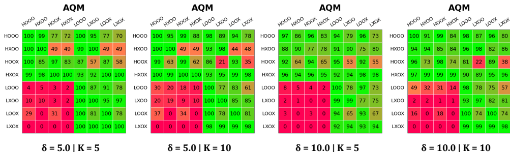
Figure 10: AQM hyperparameter sensitivity. Performance heatmaps of AQM as a function of the separation radius \delta (controls keypoint sparsity) and the subgoal sampling distance K (controls how far subgoals are sampled along trajectories). Rows denote the training environment and columns denote the evaluation environment.
