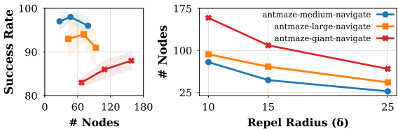
Figure 2: Performance trade-offs given \delta .
