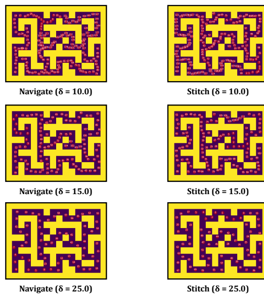
Figure 13: OGBench : Learned Mappings on Giant Maze according to the Dataset and the Repel Range ( \delta ).
