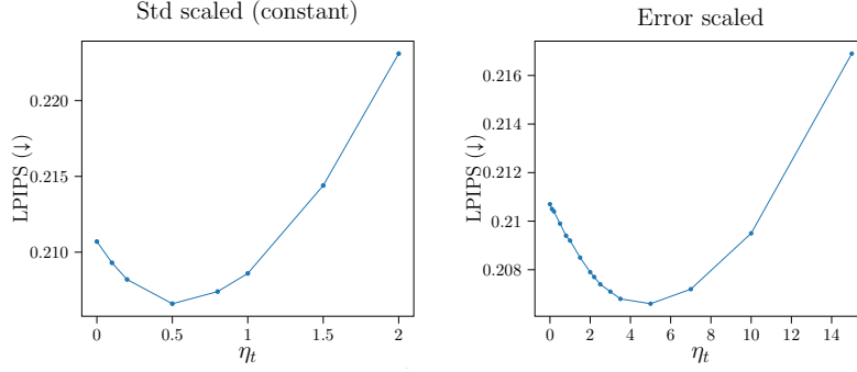
Figure 6: Effect of guidance step size on best reconstruction in terms of LPIPS. We perform experiments on the CelebA-HQ validation set on the deblurring task.
