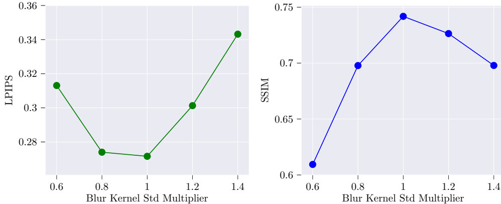
Figure 9: Effect of Gaussian blur kernel width perturbation on the FFHQ test set for the deblurring task. The change in the LPIPS metric (left) together with the SSIM metric (right) is shown.
