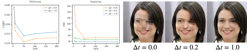
Figure 10: Effect of incremental reconstruction loss step size on the CelebA-HQ validation set for deblurring (left) and inpainting (middle). Visual comparison of inpainted samples is shown on the right.
