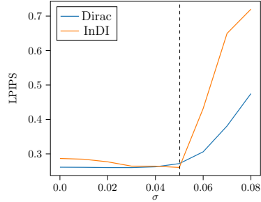
Figure 8: Robustness experiment: we simulate a mismatch between train and test noise levels (FFHQ test split, deblurring). Dirac is more robust to perturbations in measurement noise variance.
