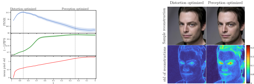
Figure 3: Perception-distortion trade-off on CelebA-HQ deblurring: distortion metrics initially improve, peak fairly early in the reverse process, then gradually deteriorate, while perceptual metrics improve. We plot the mean of 30 trajectories ( \pm std shaded) starting from the same measurement.
