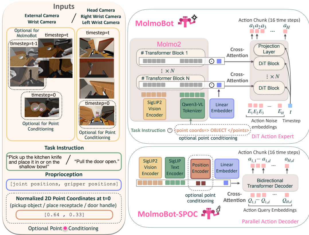
Fig. 3: Left: MolmoBot policies ingest multiple RGB camera views (from possibly multiple timesteps), proprioceptive state, and a language task instruction. Optionally, policies can be additionally conditioned on 2D points, represented as a grounding image and a point coordinate in that image. Top right: MolmoBot uses a Molmo2-4B vision-language backbone and a DiT-based flow matching action head that cross-attends to state features to denoise action chunks. Bottom right: MolmoBot-SPOC is a lightweight transformer-based policy, using a transformer decoder to predict an action chunk in parallel, conditioned on frozen SigLIP2 vision and text embeddings. MolmoBot-Pi0 (not shown) exactly follows the \pi_0 [3] architecture, initialized from PaliGemma [2] weights and a randomly initialized action expert.
