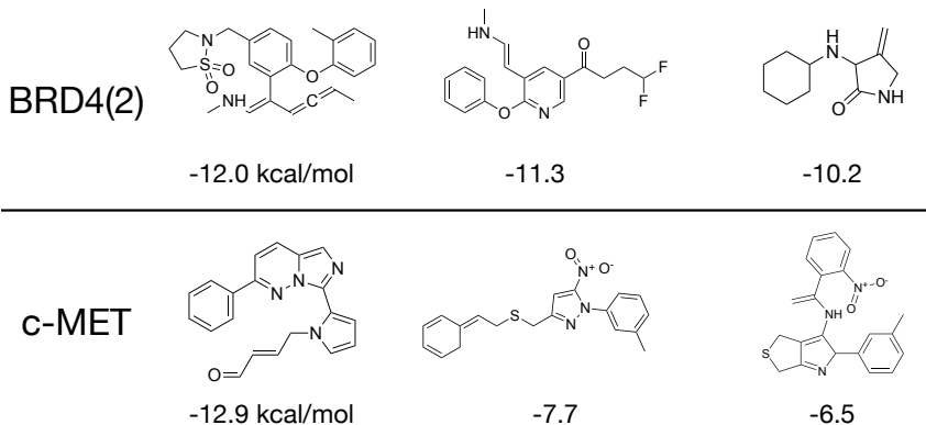
Figure 2: Visualization of MF-LAL generated molecules. The top 3 molecules and associated ABFE scores are shown for both the BRD4(2) (top row) and c-MET (bottom row) targets.
