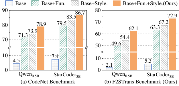
Figure 3: Model performance under different training strategies: base LLMs, function guidance (Fun.), style guidance (Style.), and our function-to-style guidance.
