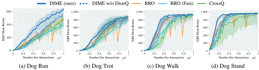
Figure 9: Ablation on Distributional Q. Comparison of DIME and DIME without employing distributional Q (dashed line). While there is a small improvement when using distributional Q, DIME w/o Distributional Q still performs on par, or better than BRO, which employs quantile distributional RL. DIME w/o DistrQ outperforms CrossQ and BRO (Fast).
