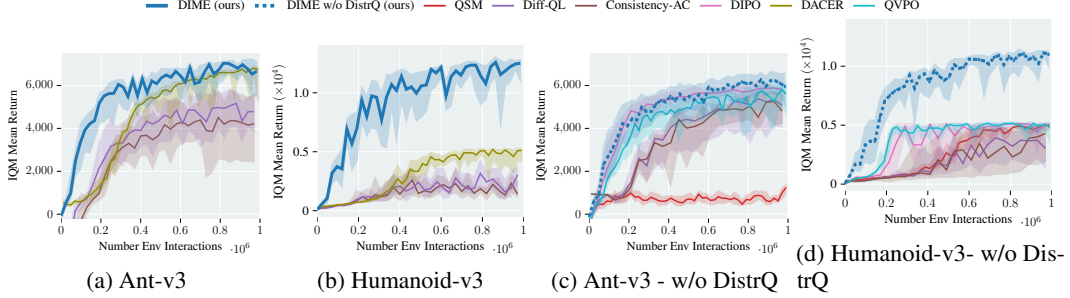
Figure 8: Comparison to Diffusion Baselines with (a-b)) and without Distributional Q (c-d)) on the Ant-v3 and Humanoid-v3 tasks. We provide the learning curves for distributional versions for Diff-QL and Consistency-AC alongside DACER, which employs distributional Q by default on the Ant-v3 (a) and Humanoid-v3 (b) tasks. DIME converges faster on the Ant-v3 (a) task to the same performance achieved by DACER and outperforms all baselines on the more high-dimensional Humanoid-v3 (b) task. Additionally, we compare DIME without distributional Q against the diffusion baselines without distributional Q on the Ant-v3 (c) and Humanoid-v3 (d) tasks. DIME without distributional Q performs on par with the baselines DIPO and QVPO on the Ant-v3 (c) and outperforms all baselines on the Humanoid-v3 (d).
