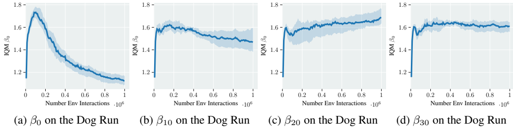
Figure 7: Learned \beta parameters. DIME’s policy improvement objective (Eq. 26) allows to train various parameters end-to-end, such as the scaling for the diffusion coefficient \beta . More concretely, we train a scaling parameter \beta_k per dimension k , that scales the cosine schedule. We visualize the adaptation of the parameter for the dimension k = 0, 10, 20, 30 over the training, averaged over 10 seeds for the dog-run task. Clearly, DIME first increases the parameter at the beginning of the training phase. Depending on the dimension, it either converges to a rather high value ( k = 20 and k = 30 ), or keeps being reduced for other dimensions k = 0 and k = 10 .
