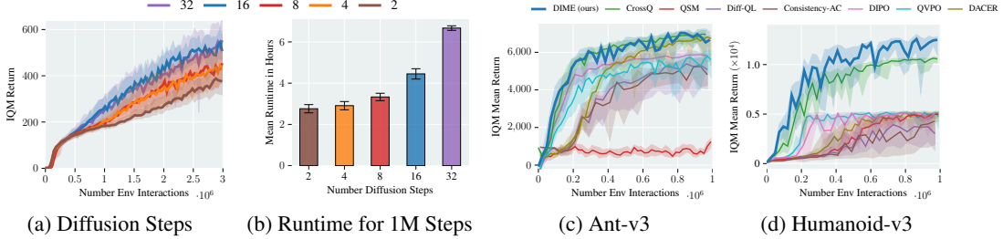
Figure 3: Varying the Number of diffusion steps (a)-(b). The number of diffusion steps might affect the performance and the computation time. (a) shows DIME’s learning curves for varying diffusion steps. Two diffusion steps perform badly, whereas four and eight diffusion steps perform similar but still worse than 16 and 32 diffusion steps which perform similarly. (b) shows the computation time for 1MIO steps of the corresponding learning curves. The smaller the diffusion steps, the less computation time is required. Learning Curves on Gym Benchmark Suite (c)-(d). We compare DIME against various diffusion baselines and CrossQ on the (c) Ant-v3 and (d) Humanoid-v3 from the Gym suite. While all diffusion-based methods are outperformed by DIME, DIME performs on par with CrossQ on the Ant environment. DIME performs favorably on the high-dimensional Humanoid-v3 environment, where it also outperforms CrossQ.
