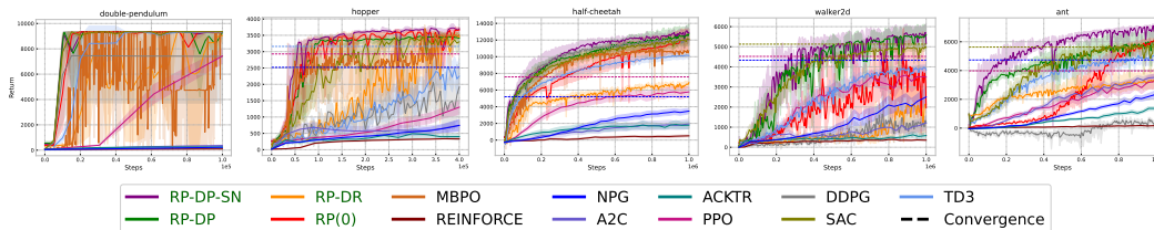
Figure 1: Comparisons between RP PGMs (the green labels) and MF/MB baselines (the black labels) in the MuJoCo [57] tasks.
