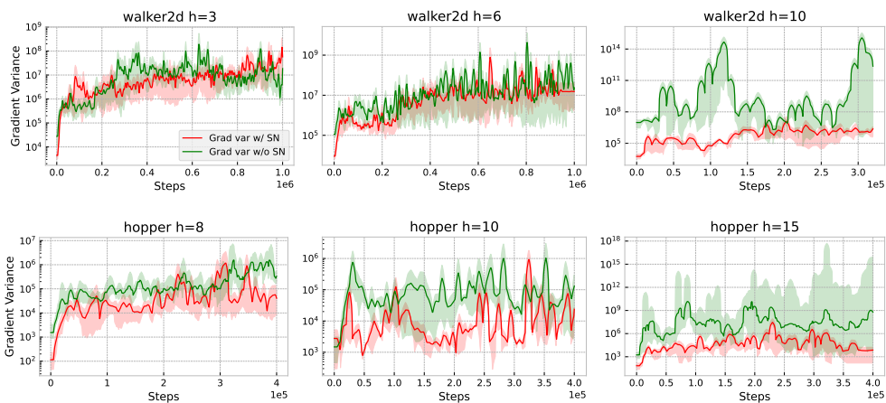
Figure 13: Gradient variance of RP PGMs. The variance is significantly lower with SN when h is large.
