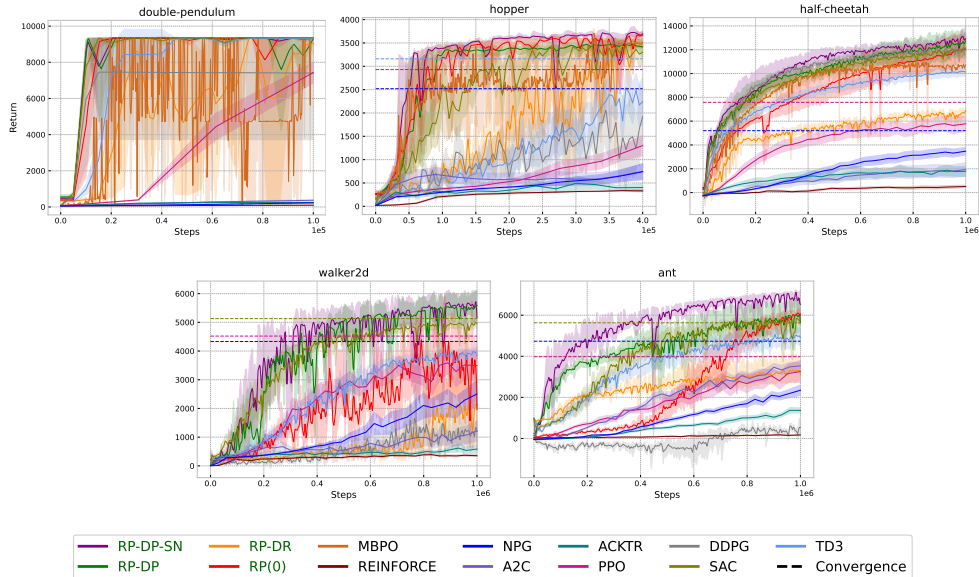
Figure 11: Comparisons between RP PGMs (the green labels) and MF/MB baselines (the black labels) in the MuJoCo [57] tasks.
