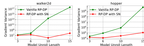
Figure 2: Gradient variance of the vanilla RP-DP explodes while adding spectral normalization solves this issue.
