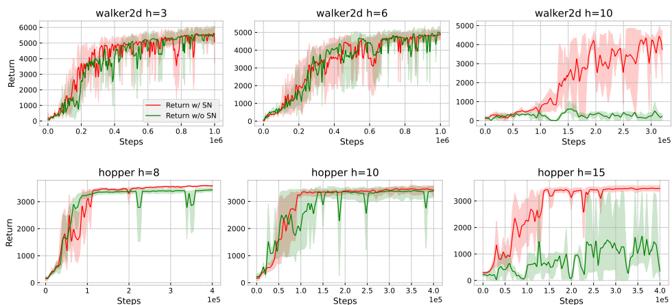
Figure 12: Performance of vanilla and SN-based MB RP PGMs with varying h . The vanilla method only works with a small h and fails when h increases, while the SN-based method enables a larger h .
