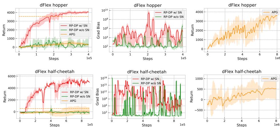
Figure 14: Performance and gradient bias in differentiable simulation. The last column is the full training curves of APG, which need 20 times more steps than RP-DP-SN to reach a comparable return in the hopper task and fail in the half-cheetah task, respectively.
