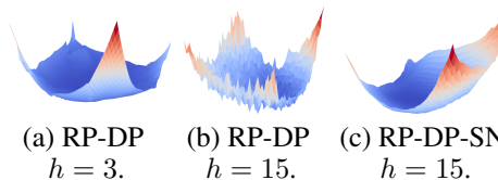
Figure 3: The loss surface of hopper.
