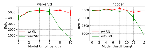
Figure 5: Performance with different h .
