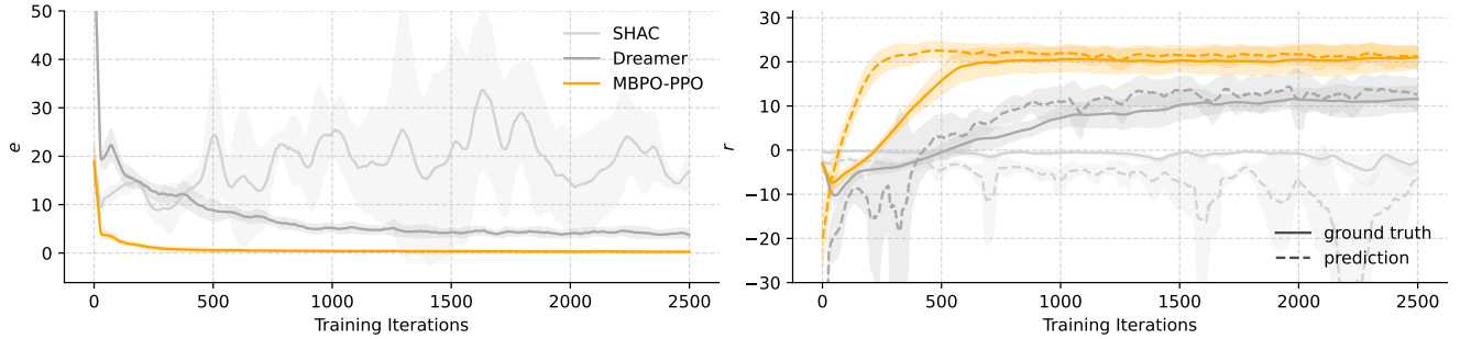
Figure 3. Model error and policy mean reward for the ANYmal D velocity tracking task with MBPO-PPO. The policy is trained using estimated rewards computed from predicted observations by RWM. Ground truth rewards, visualized with solid lines, are reported by the simulator for evaluation purposes only.
