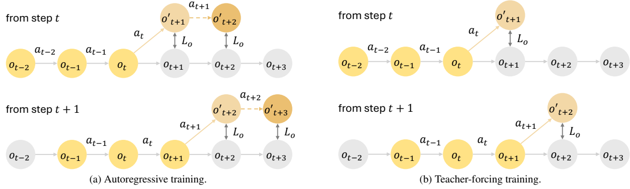
Figure S5. Comparison of training paradigms for world models with an example of a history horizon H = 3 . (a) Autoregressive training operates with an example of a forecast horizon N = 2 , leveraging historical data and its own predictions for long-horizon robustness. The dashed arrows denote the sequential autoregressive prediction steps. (b) Teacher-forcing training can be viewed as a special case of autoregressive training with a forecast horizon N = 1 , using ground truth observations for next-step predictions to optimize parallelization but limiting robustness to error accumulation.
