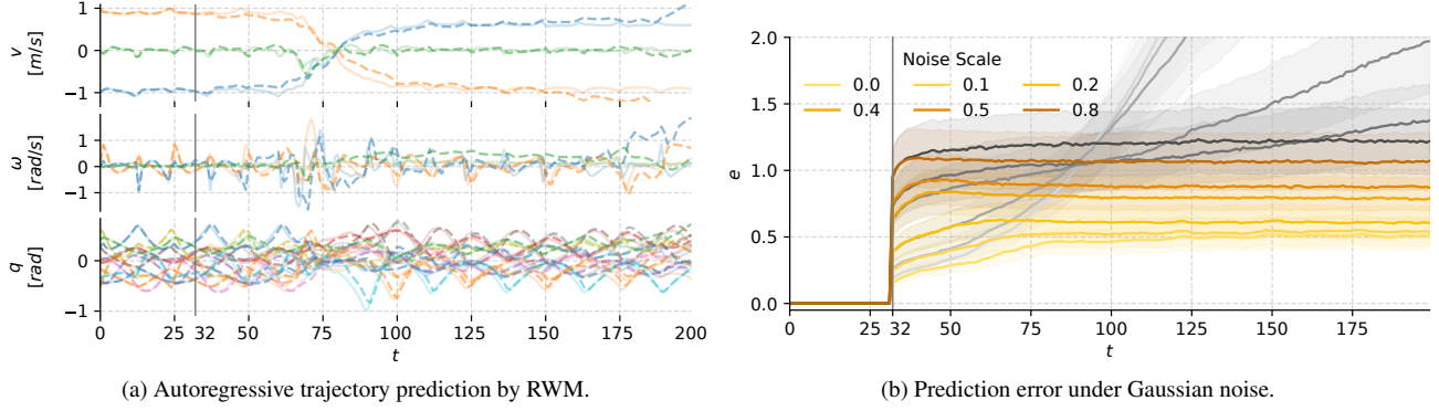
Figure S4. (Left) Solid lines represent ground truth trajectories, while dashed lines denote predicted state evolution. Predictions commence at t = 32 using historical observations, with future observations predicted autoregressively by feeding prior predictions back into the model. (Right) Yellow curves denote RWM at varying noise levels, demonstrating consistent robustness and lower error accumulation across forecast steps. Grey curves represent the MLP baseline, which exhibits significantly higher error accumulation and reduced robustness to noise.
