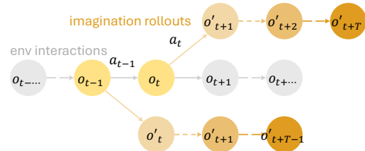
Figure S7. Model-Based Policy Optimization with learned world models. The framework combines real environment interactions with simulated rollouts for efficient policy optimization. Observation and action pairs from the environment are stored in a replay buffer and used to train the autoregressive world model. Imagination rollouts using the learned model predict future states over a horizon of T , providing trajectories for policy updates through reinforcement learning algorithms.
