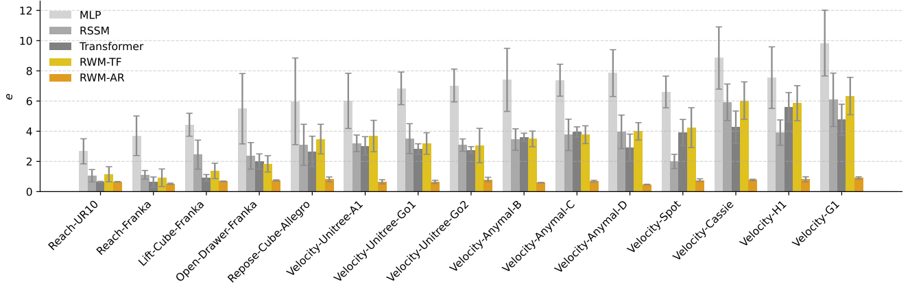
Figure 2. Autoregressive trajectory prediction errors across diverse robotic environments and network architectures. RWM trained with autoregressive training (RWM-AR) consistently outperforms baseline methods, including MLP, recurrent state-space model (RSSM), and transformer-based architectures. RWM-AR demonstrates superior generalization and robustness across tasks, from manipulation to locomotion. Autoregressive training (RWM-AR) reduces compounding errors over long rollouts, significantly improving performance compared to teacher-forcing training (RWM-TF).
