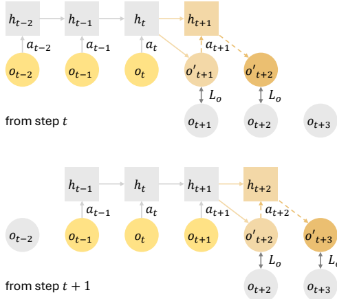
Figure S6. Dual-autoregressive mechanism employed in RWM. Inner autoregression updates GRU hidden states after each historical step within the context horizon, while outer autoregression feeds predicted observations from the forecast horizon back into the network. The dashed arrows denote the sequential autoregressive prediction steps, highlighting robustness to long-term dependencies and transitions.
