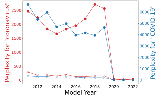
Figure 1: The perplexity of coronavirus and COVID-19 , using TiMaGPT models (•) and Conventional Temporally Adapted (CTA) models (×). The calculation for perplexity is outlined in Appendix H and the methodology for temporally adapting models is explained in Section 5. The CTA models have significant knowledge of these words before the pandemic.
