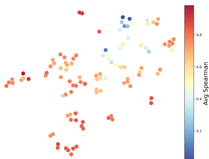
Figure 5: Submap of 112 encoders coloured by the average Spearman correlation between the true and predicted task performance of selected tasks.
