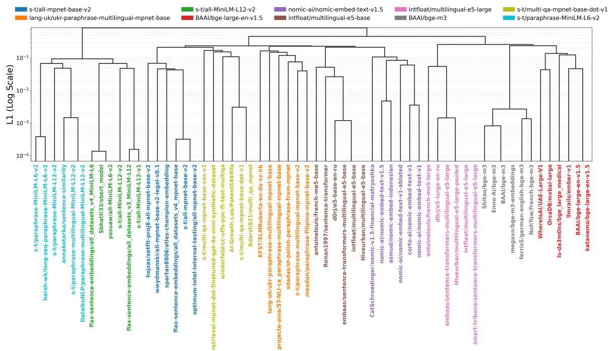
Figure 6: Heirarchical Clustering for 10 randomly selected encoders with top 5 nearest neighbours.
