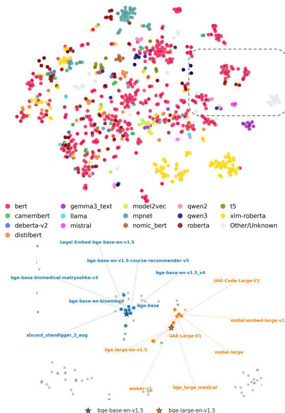
Figure 1: Map of Encoders. Top: Map for 1101 sentence encoders, visualised by t-SNE and coloured by the encoder type. Bottom: A 30% zoomed-in view of the dotted area showing the top-7 nearest neighbours for bge-base and bge-large . We see that the nearest neighbours belong to the same primary architecture and are closely located.
