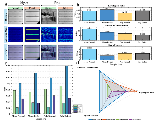
Fig. 8. Attention pattern analysis of SCRViT model using GradCAM. (a) Attention visualization results for different sample types, including normal and defective samples of mono- and poly-crystalline PV modules. Each group displays, from top to bottom, the original EL image, attention heatmap, and overlay image. The heatmap colors range from blue to red, indicating low to high attention intensity. (b) Quantitative analysis of three key metrics: Key Region Ratio reflecting the relative size of attended areas, Attention Concentration characterizing the degree of focus, and Spatial Variance describing the uniformity of attention distribution. (c) Comparison of basic statistical features across sample types, including Mean, Standard Deviation (Std), Maximum (Max), and Minimum (Min). (d) Radar chart analysis showing comprehensive performance characteristics across three dimensions for different sample types, with blue, red, green, and purple representing mono-crystalline normal, mono-crystalline defective, poly-crystalline normal, and poly-crystalline defective samples, respectively.
