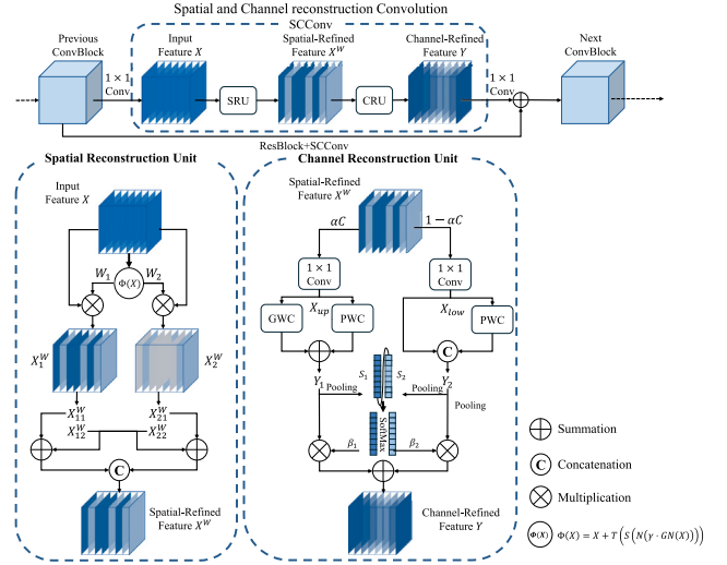
Fig. 3. Schematic diagram of the SCConv module and its subunit structure. The module consists of two functional units, SRU and CRU, which enhance the model's feature extraction capability for non-uniform EL images through feature separation, reconstruction, and adaptive fusion operations.
