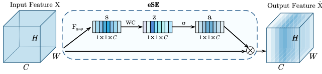
Fig. 4. Architecture of the ESE module. The module performs feature recalibration through global average pooling for channel statistics extraction, followed by channel relationship modeling and Sigmoid activation for attention weight generation.
