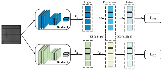
Fig. 5. Example of Deep Mutual Learning (DML) strategy with dual networks. The figure illustrates the mutual learning process between networks \Theta_1 and \Theta_2 , where each network is trained using supervised learning loss and Kullback–Leibler divergence-based mimicry loss. This framework naturally extends to collaborative training scenarios with multiple networks, enabling multi-directional knowledge transfer.
