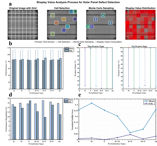
Fig. 7. Feature attribution analysis based on Shapley values. (a) Four-stage computation pipeline: original image grid partitioning ( 8 \times 8 ), feature unit selection, Monte Carlo sampling ( M = 1000 ), and Shapley value heatmap generation, where red regions indicate areas with high contribution to model predictions; (b) Comparative impact of different perturbation types on mono- and poly-crystalline modules, with bar heights showing mean impact and error bars indicating standard deviation ( \pm 1\sigma ); (c) Response ranges of mono-crystalline (left) and poly-crystalline (right) modules under various environmental perturbations, with y-axis showing response percentage (0%–100%) and vertical lines indicating min–max response range; (d) Performance degradation percentage analysis under environmental factors; (e) Normalized model stability score trends, computed through inverse standardization of response standard deviations. Here, B (Brightness), M (Motion Blur), and P (Posterize) represent illumination variation ( \pm 0.5 ), motion blur (kernel size = 7), and temperature-induced image quality degradation (bit depth = 7), respectively.
