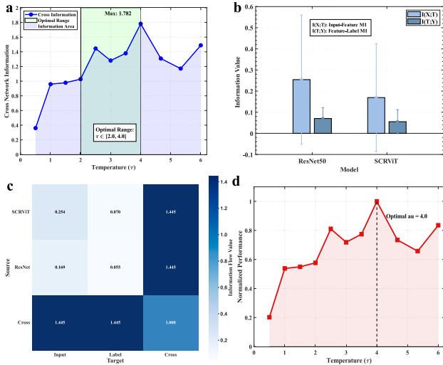
Fig. 9. Information-theoretic analysis of deep mutual learning. (a) Effect of temperature parameter \tau on inter-network mutual information I(T_1; T_2) ; (b) Comparison of feature-input mutual information I(X; T) and feature-label mutual information I(T; Y) between SCRvIT and ResNet-50; (c) Information flow matrix showing network interaction strength; (d) Normalized performance curve with respect to temperature \tau .
