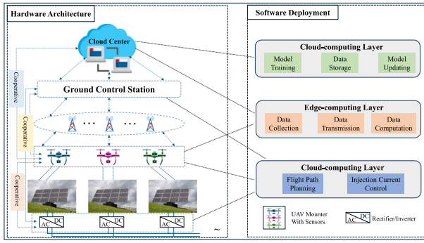
Fig. 1. Architecture of IoT-based EL image defect detection system. The hardware layer integrates cloud computing centers, ground stations, and drone swarms. The software layer implements end-to-end deployment from data acquisition to model training. (For interpretation of the references to color in this figure legend, the reader is referred to the web version of this article.)
