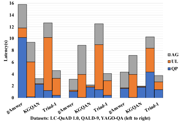
Figure 3: Response time of traditional KBQA systems and Triad on three datasets. Each bar shows average response time of a particular phase of KBQA.
