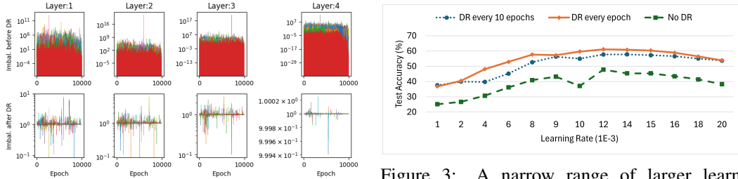
Figure 3: A narrow range of larger learning rates results in better generalization for roman-empire dataset on GAT, with further improvement brought by dynamic rescaling (DR) to balance relative gradients.
