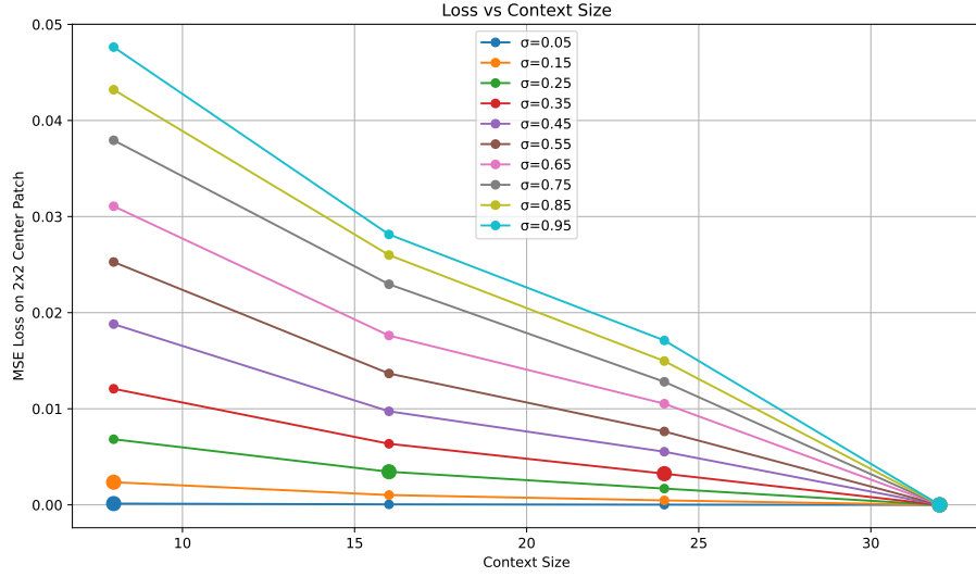
Figure 11: ImageNet-512x512: denoising loss of an optimally trained model, measured at 2 \times 2 center patch, as we increase the context size given to the model (horizontal axis) and the noise level (different curves). As expected, for higher noise, more context is needed for optimal denoising. The large dot on each curve marks the point where the loss nearly plateaus.
