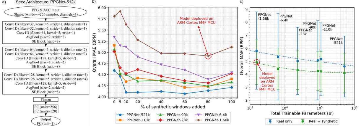
Fig. 2. a) PPGNet-512. b), c) Synthetic augmentation to improve test MAE maintaining pareto efficiency
