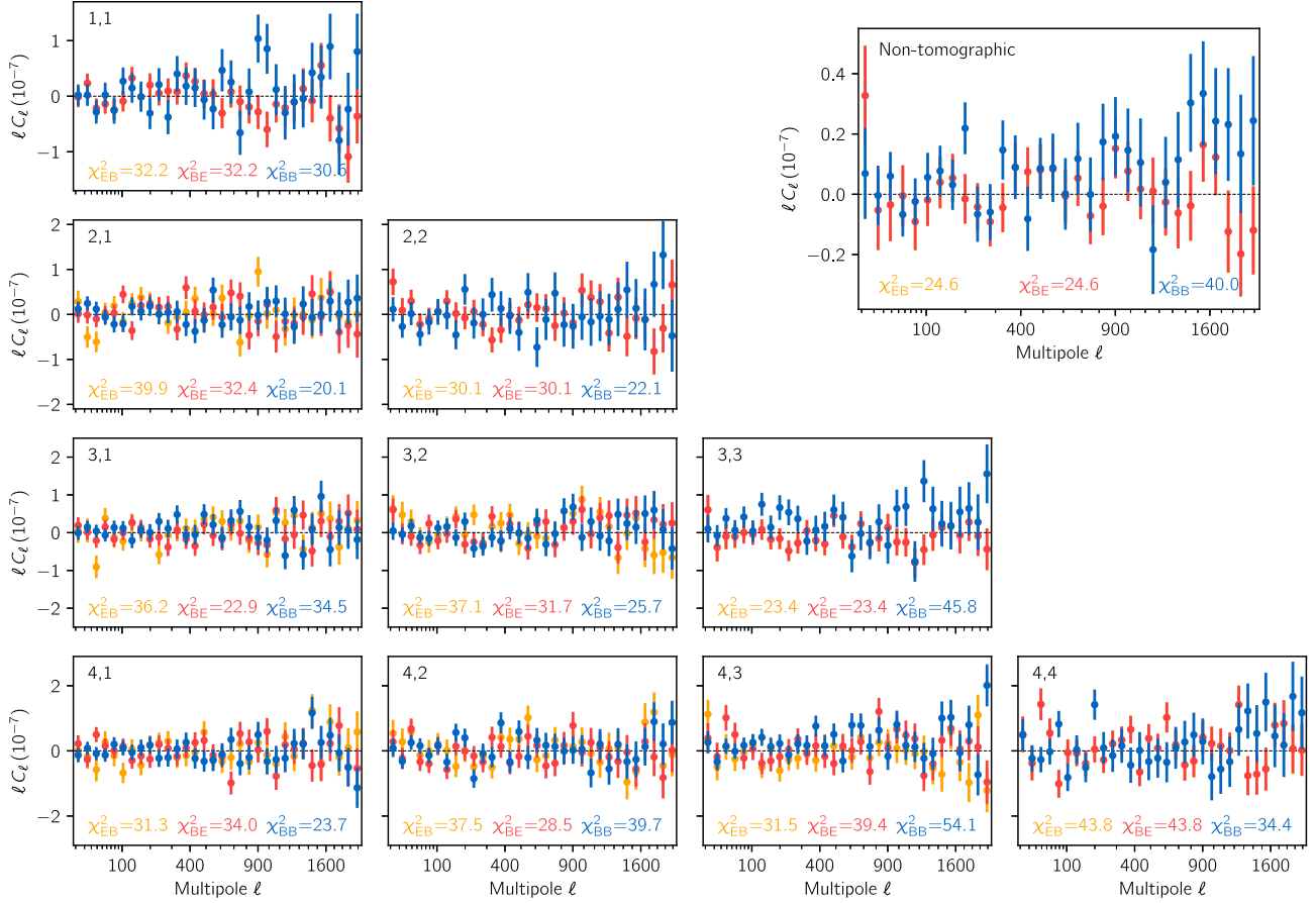
Figure 8. EB and BB cosmic shear power spectra measured with DES Y3 data for each pair of tomographic bins in the lower triangle, and the entire sample in the upper right panel (note that the EB and BE power spectra are different only for cross-redshift bin spectra). Error bars are computed from 10 000 Gaussian simulations using the DES Y3 catalog ellipticities and positions, as explained in Section 4.1.1. We find a \chi^2 of 344.0 for 320 degrees of freedom for tomographic B -mode power spectra, corresponding to a probability-to-exceed of 0.17. We find a \chi^2 of 535.4 for 512 degrees of freedom for EB tomographic cross-power spectra (counting all 16 independent bin pairs), corresponding to a probability-to-exceed of 0.23. Individual \chi^2 are reported for each redshift bin pairs in the corresponding panels. In the non-tomographic case, we find, for the B -mode power spectrum, a \chi^2 of 40.0 for 32 degrees of freedom, corresponding to a probability-to-exceed of 0.16.
