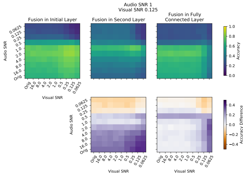
Figure 12: Late fusion model where audio SNR = 1, and visual SNR = 0.125. Fusion in the initial layer outperforms the fusion in the fully connected layer for audio SNR values greater than 1.
