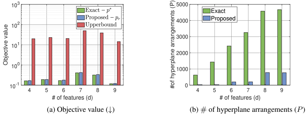
Figure 4: Verification of Theorem 2 and Remark 2. We train a parallel network using the convex program in Theorem 1 with \ell_2 loss on a toy dataset with n = 15 , \beta = 0.1 , m_2 = 1 , and the low-rank approximation r = \lfloor \frac{d}{2} \rfloor . To obtain a low-rank model, we first sample a data matrix from a standard normal Gaussian distribution and then set \sigma_{r+1} = \dots = \sigma_d = 1 .
