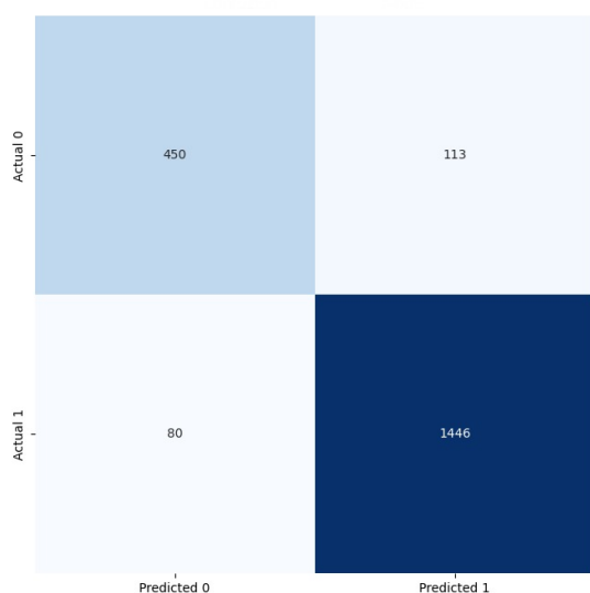
Fig. 2. Confusion matrix of SVM(1-3 Feature).
