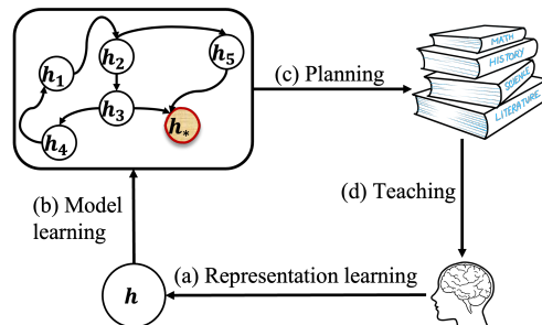
Figure 1: The teaching framework. Our work focuses on steps (b), (c) and (d), and assumes the feature mapping (i.e. learned through step (a)) is known and given.
