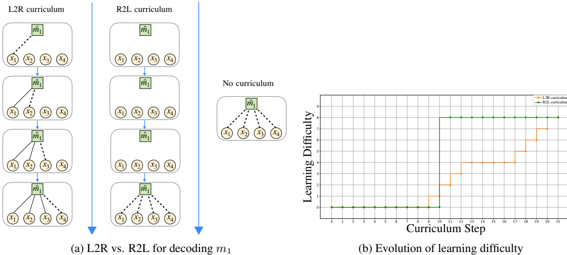
Figure 6: L2R vs. R2L: (a) Bit estimates evolve more smoothly under L2R than R2L for Polar(4, 4), (b) Learning difficulty increases more gracefully for L2R than R2L for Polar(64, 22).
