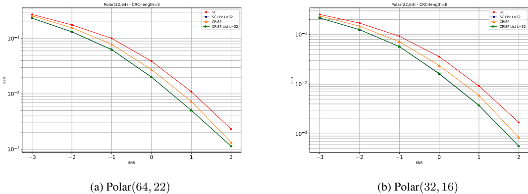
Figure 18: CRISP performs well on CRC-Polar code
