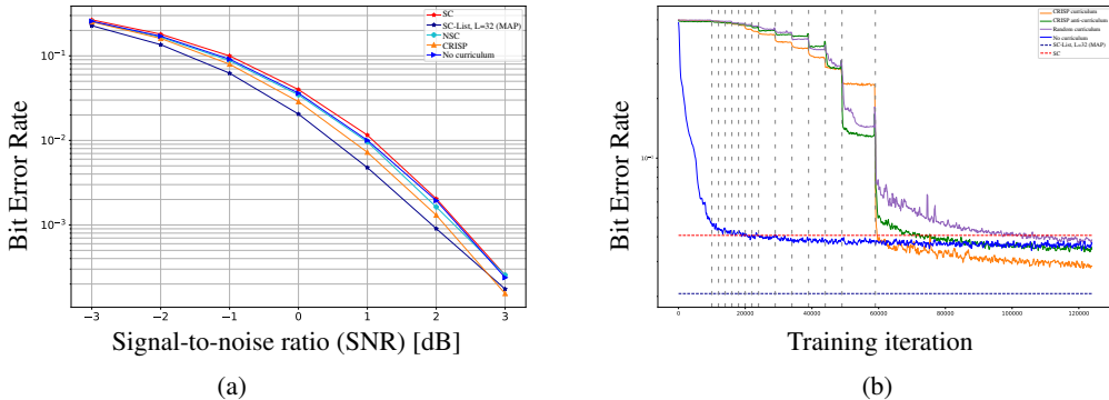
Figure 1: (a) CRISP achieves near-MAP reliability for Polar(64, 22) code on the AWGN channel. (b) Our proposed curriculum is crucial for the gains CRISP attains over the baselines; details in Sec. 4.
