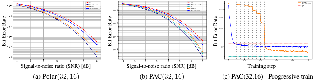
Figure 5: CRISP outperforms baselines and attains near-MAP performance for Polar(32, 16) and PAC(32, 16) codes on the AWGN channel.
