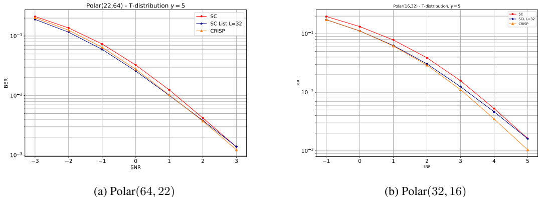
(a) Polar(64, 22) (b) Polar(32, 16) Figure 17: CRISP matches SCL reliability on T-distributed channels
