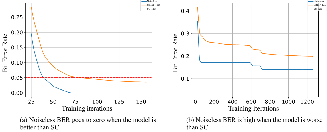
Figure 7: Evolution of training BER at 1dB and noiseless BER for CRISP.
