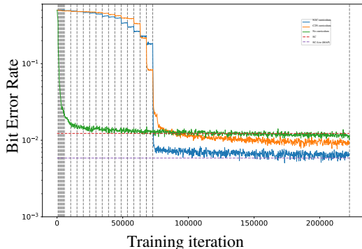
Figure 15: L2R curriculum helps CNN to achieve near-optimal reliability
