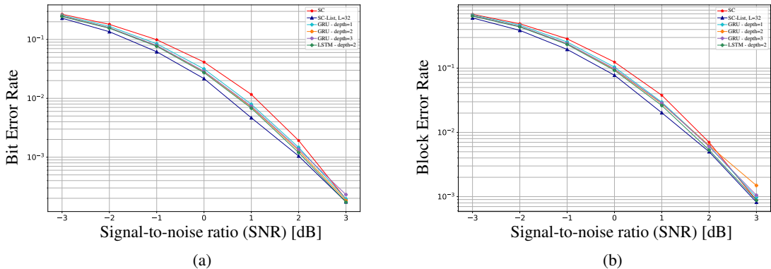
Figure 22: Polar(64, 22): LSTMs and GRUs achieve similar reliability.
