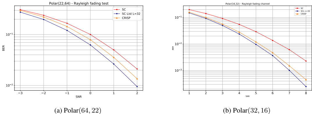
(a) Polar(64, 22) (b) Polar(32, 16) Figure 16: CRISP achieves good reliability on Rayleigh fading channels
