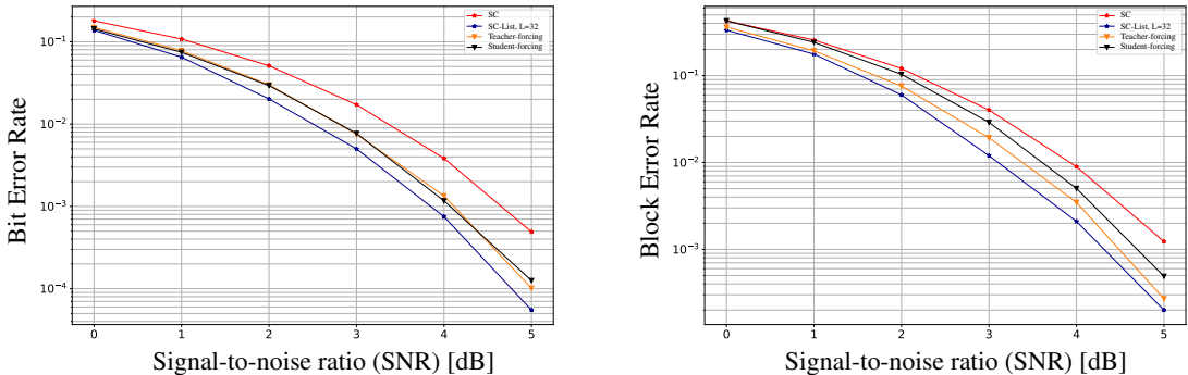
Figure 23: Training CRISP using student forcing results in sub-optimal BLER.
