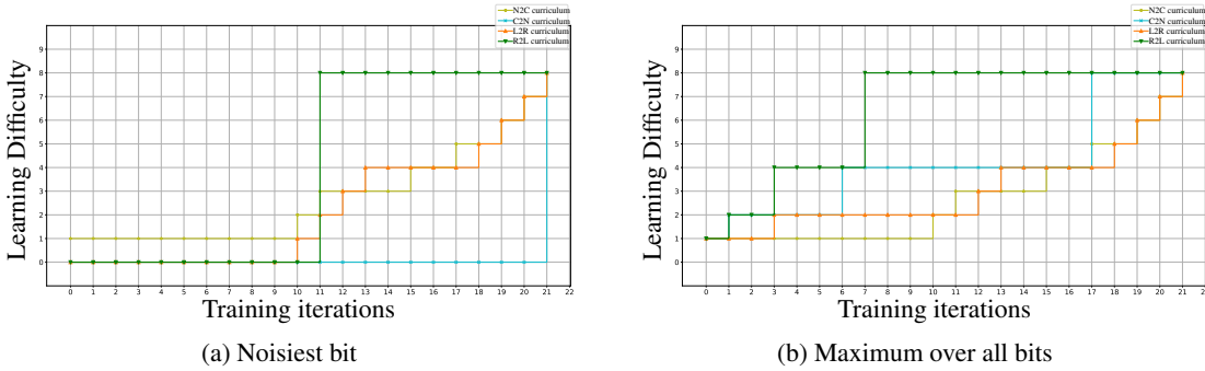
Figure 12: Evolution of learning bit difficulty for different curricula for Polar(64, 22).
