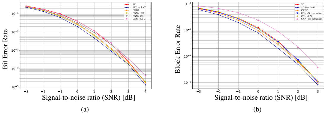
Figure 14: a) CNN decoder achieves near-MAP BER performance with L2R curriculum. b) CRISP achieves near-MAP BLER for Polar(64, 22). CNN is slightly worse.
