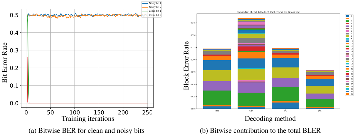
Figure 8: Error analysis for Polar(64, 32) : (a) Noiseless BER for the two least reliable bits gets stuck at 0.5 whereas it converges to 0 for the two most reliable bits, (b) Contribution of each bit (conditioned on no previous errors) to the BLER.
