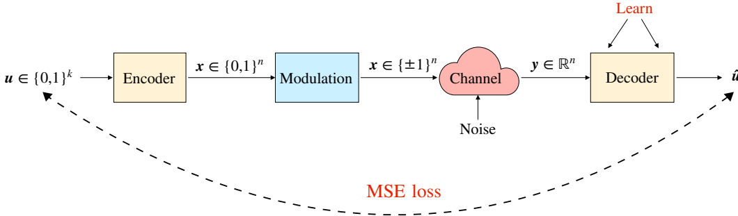
Figure 2: Channel decoding problem.
