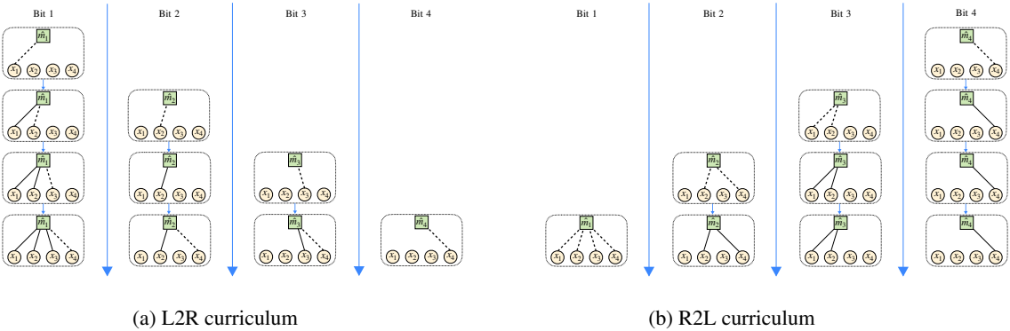
Figure 9: Evolution of the MAP decoding rules for L2R and R2L for Polar(4, 4). Dotted lines indicate new coded bits being introduced into the decoding rule at each curriculum step.
