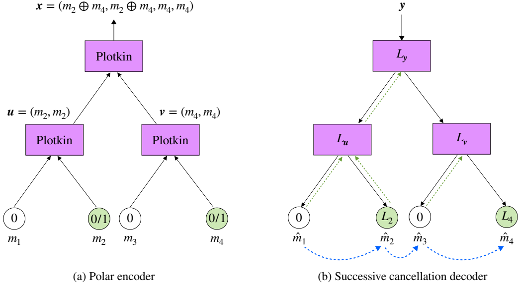
Figure 3: Polar(4, 2): (a) Polar encoding via Plotkin tree; (b) Blue arrows indicate the decoding order.
