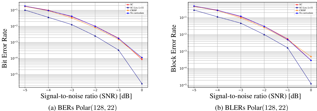
Figure 21: CRISP matches SC reliability on Polar(128, 22).
