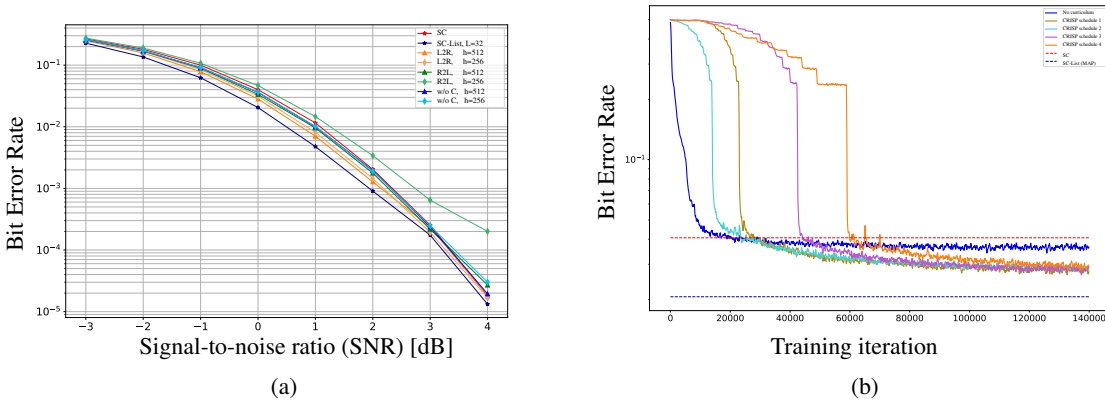
Figure 13: Ablation plots: (a) Choosing the right curriculum is critical when model size is smaller, (b) The number of iterations to train CRISP on each subcode using the L2R/N2C curriculum are not critical to the final performance achieved.
