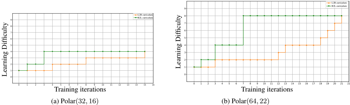
Figure 10: Evolution of the learning difficulty for L2R and R2L.
