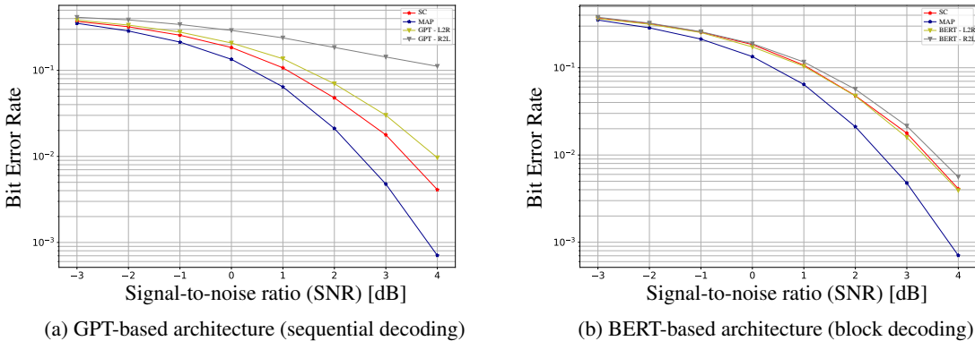
Figure 19: Transformer performance on Polar(32, 16).
