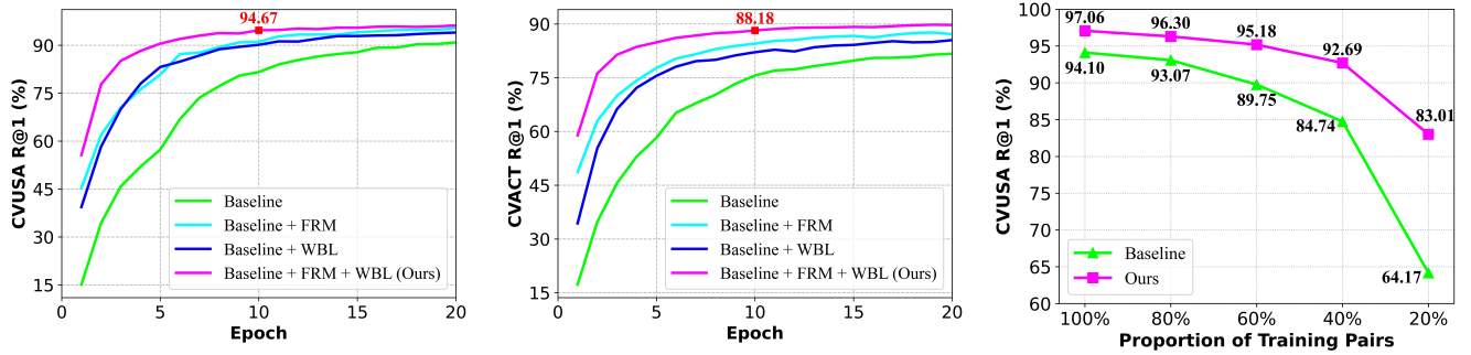
Figure 4: Left and Middle: The training curve (R@1) on CVUSA (Left) and CVACT (Middle) datasets. The red dot data indicates the performance of FRGeo (Ours) at the 10th training epoch. Right: Few-shot training on CVUSA dataset. 100% indicates using all training samples. Best viewed on screen with zoom-in.
