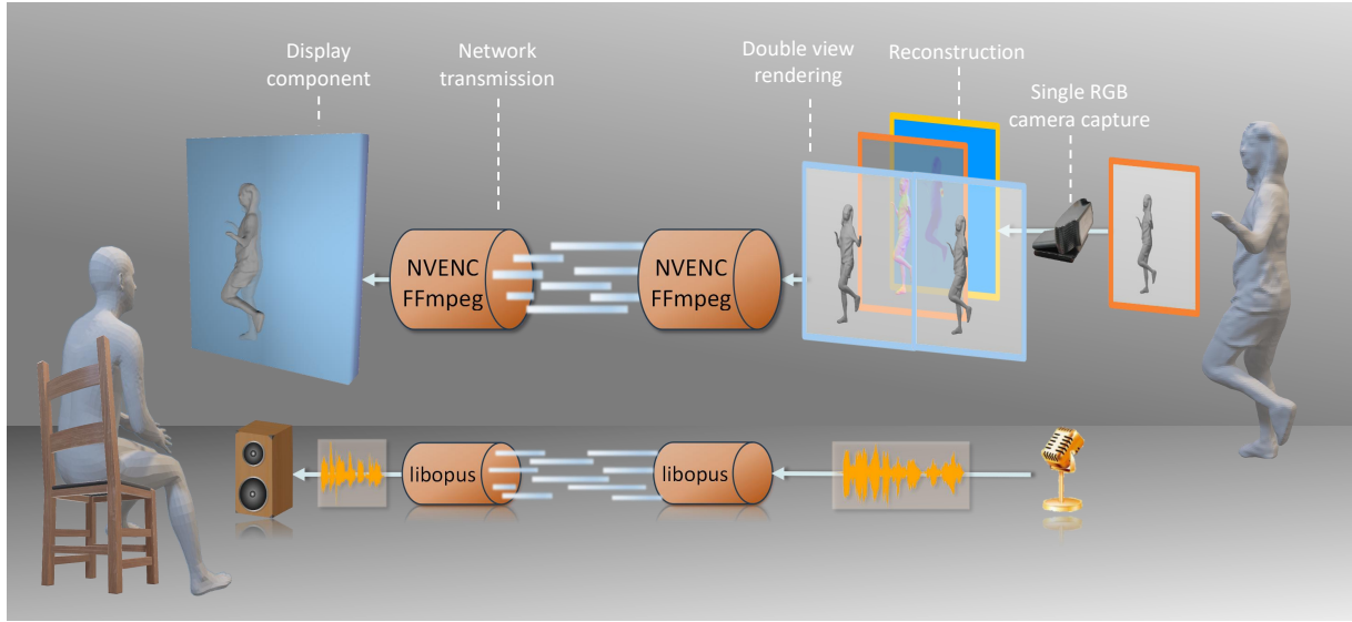
Figure 2: Schematic diagram of the overall system. We only use one USB webcam for video capture, and then perform high-quality human geometry reconstruction and double view rendering. Finally, the results are transmitted over the network to the display component for display to the user.
