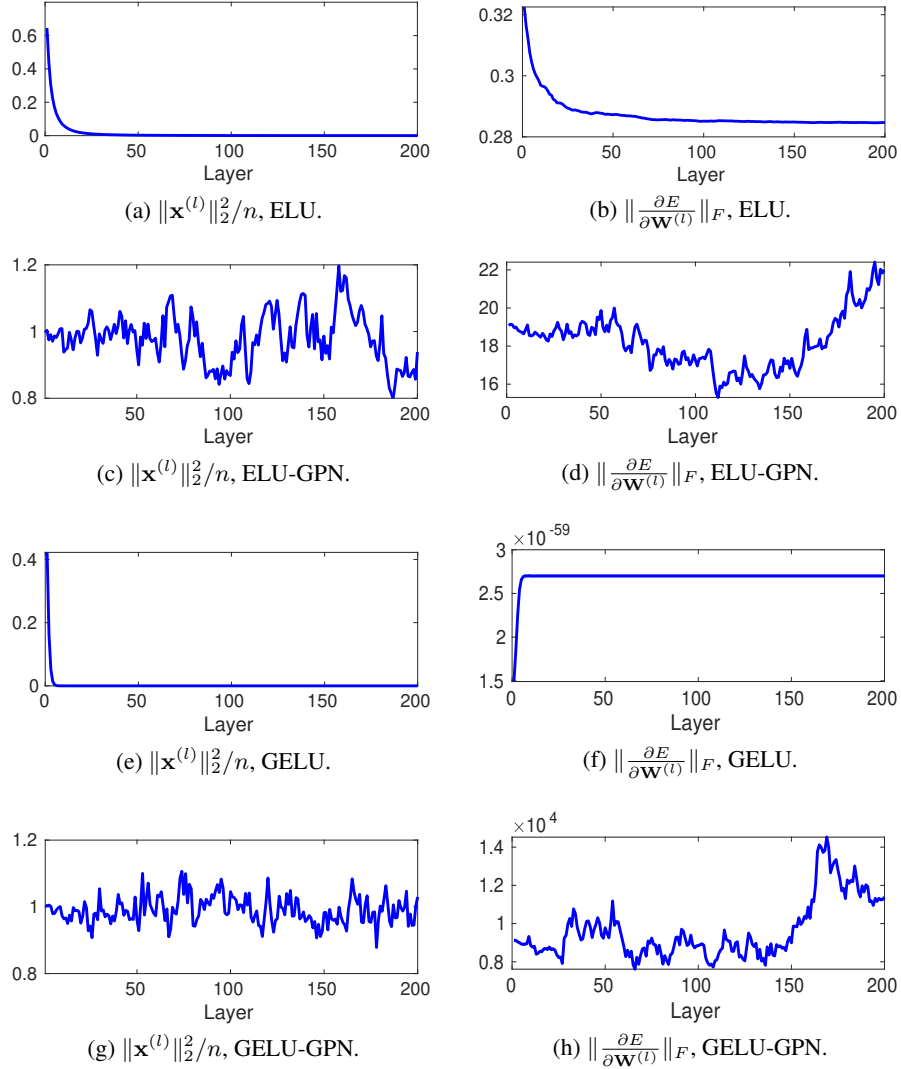
Figure 5: Results on synthetic data with different activation functions. “-GPN” denotes the function is Gaussian-Poincaré normalized. \|\mathbf{x}^{(l)}\|_2 denotes the l_2 norm of the outputs of the l -th layer. n denotes the width. \|\frac{\partial E}{\partial \mathbf{W}^{(l)}}\|_F is the Frobenius norm of the gradient of the weight matrix in the l -th layer.
