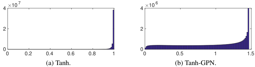
Figure 2: Histogram of \phi'(h_i^{(l)}) . The values of \phi'(h_i^{(l)}) are accumulated for all units, all layers and all samples in the histogram.
