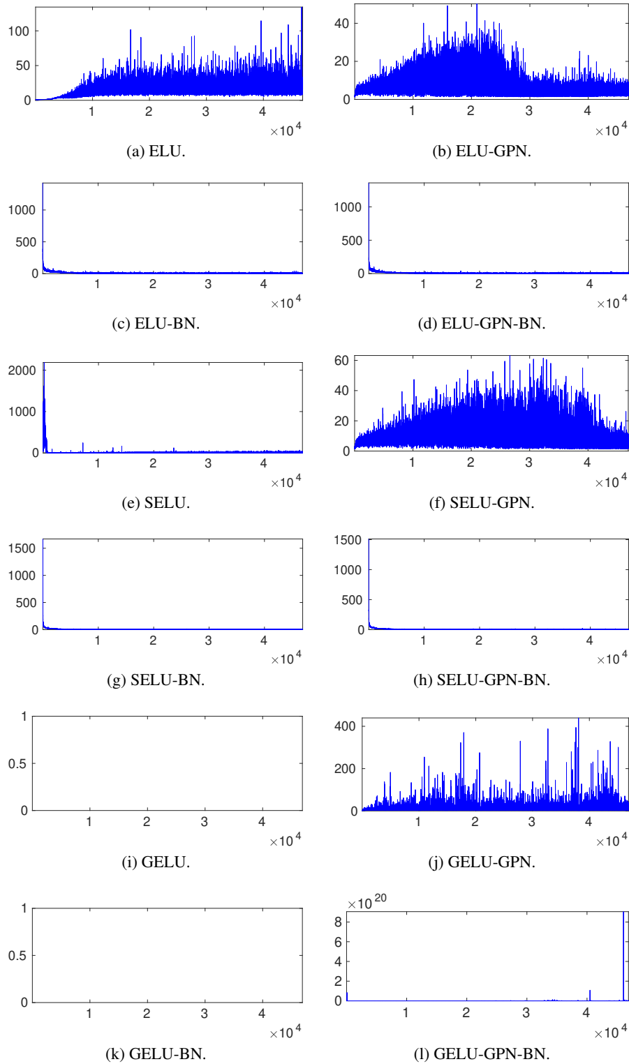
Figure 11: Gradient norm ratio during training on MNIST. Horizontal axis denotes the mini-batch updates. Vertical axis denotes the gradient norm ratio \max_l \|\frac{\partial E}{\partial \mathbf{V}^{(l)}}\|_F / \min_l \|\frac{\partial E}{\partial \mathbf{V}^{(l)}}\|_F . The gradient vanishes ( \|\frac{\partial E}{\partial \mathbf{V}^{(l)}}\|_F \approx 0 ) for GELU and GELU-BN during training and hence the plots are empty.
