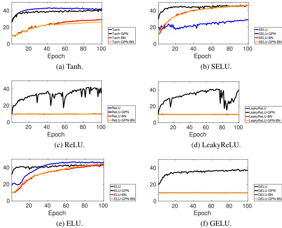
Figure 9: Test accuracy (percentage) during training on CIFAR-10.
