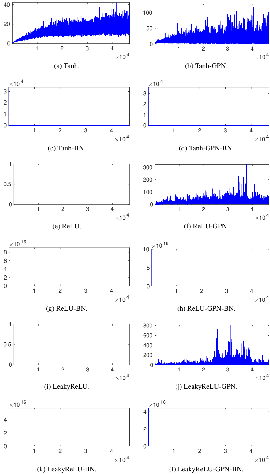
Figure 10: Gradient norm ratio during training on MNIST. Horizontal axis denotes the mini-batch updates. Vertical axis denotes the gradient norm ratio \max_l \|\frac{\partial E}{\partial \mathbf{V}(l)}\|_F / \min_l \|\frac{\partial E}{\partial \mathbf{V}(l)}\|_F . The gradient vanishes ( \|\frac{\partial E}{\partial \mathbf{V}(l)}\|_F \approx 0 ) for ReLU and LeakyReLU during training and hence the plots are empty.
