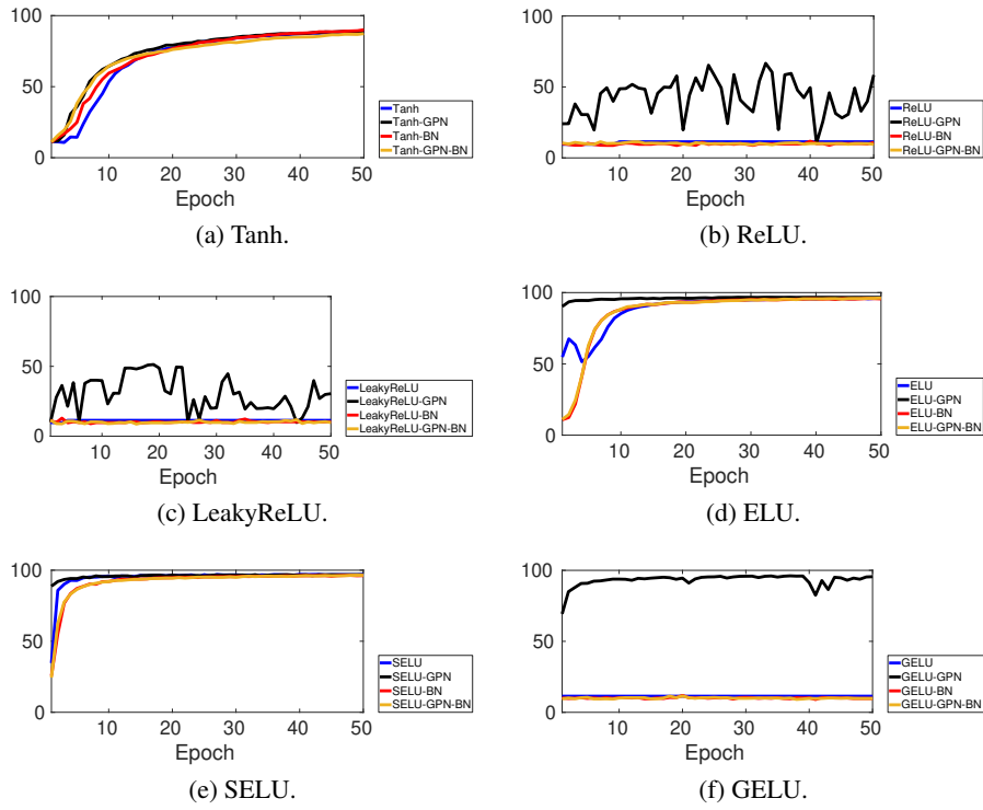
Figure 8: Test accuracy (percentage) during training on MNIST.
