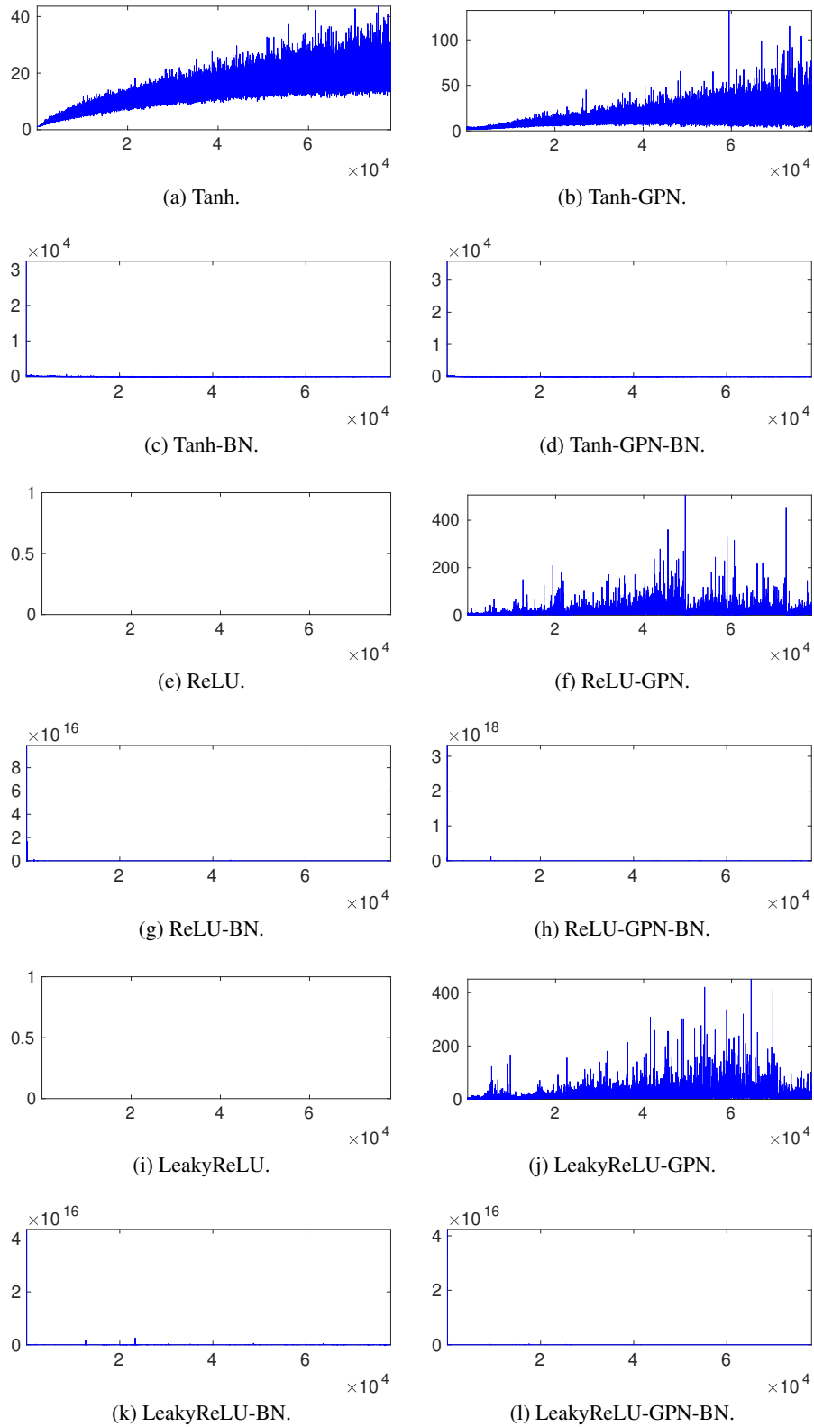
Figure 12: Gradient norm ratio during training on CIFAR-10. Horizontal axis denotes the mini-batch updates. Vertical axis denotes the gradient norm ratio \max_l \|\frac{\partial E}{\partial \mathbf{V}^{(l)}}\|_F / \min_l \|\frac{\partial E}{\partial \mathbf{V}^{(l)}}\|_F . The gradient vanishes ( \|\frac{\partial E}{\partial \mathbf{V}^{(l)}}\|_F \approx 0 ) for ReLU and LeakyReLU during training and hence the plots are empty.
