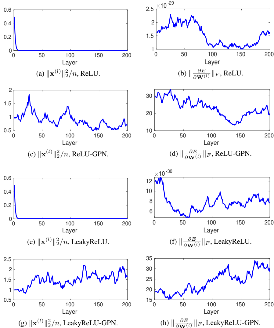
Figure 4: Results on synthetic data with different activation functions. “-GPN” denotes the function is Gaussian-Poincaré normalized. \|\mathbf{x}^{(l)}\|_2 denotes the l_2 norm of the outputs of the l -th layer. n denotes the width. \|\frac{\partial E}{\partial \mathbf{W}^{(l)}}\|_F is the Frobenius norm of the gradient of the weight matrix in the l -th layer.
