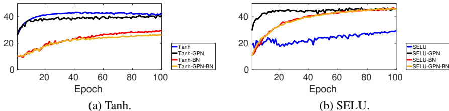
Figure 3: Test accuracy (percentage) during training on CIFAR-10. “-BN” denotes that batch normalization is applied before the activation function.
