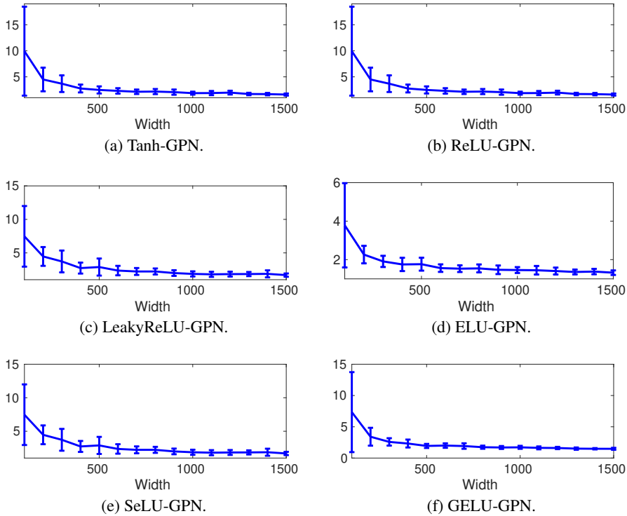
Figure 7: Gradient norm ratio for different layer width on synthetic data. The ratio is defined as \max_l \|\frac{\partial E}{\partial \mathbf{W}^{(l)}}\|_F / \min_l \|\frac{\partial E}{\partial \mathbf{W}^{(l)}}\|_F . The width ranges from 100 to 1500. The error bars show standard deviation.
