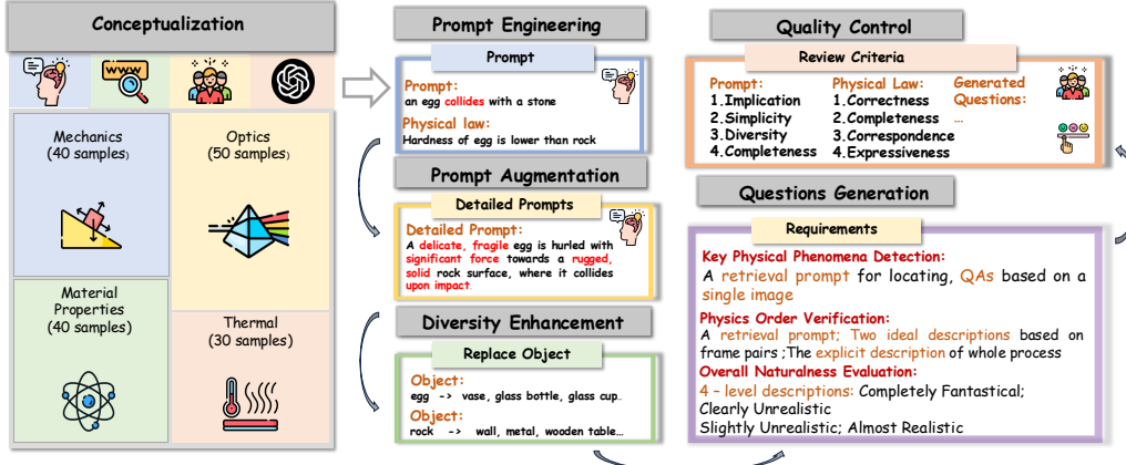
(b) The data construction pipeline of the PhyGenBench
