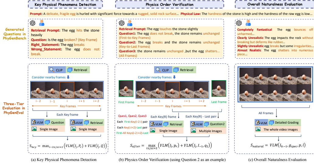
Figure 3: An overview of the proposed PhyGenEval . PhyGenEval is divided into three parts: Key Physical Phenomena Detection, Physics Order Verification, and Overall Naturalness Evaluation. Each part uses an appropriate VLM in combination with physical-based customized questions generated by GPT-4o. The final score is the combined result of the three parts. For the example in the figure, the three-stage scores are 0, 1 (only Question 1 is correct), and 0. The final score is calculated as 0 according to Overall Score calculation in Section 4.2.
