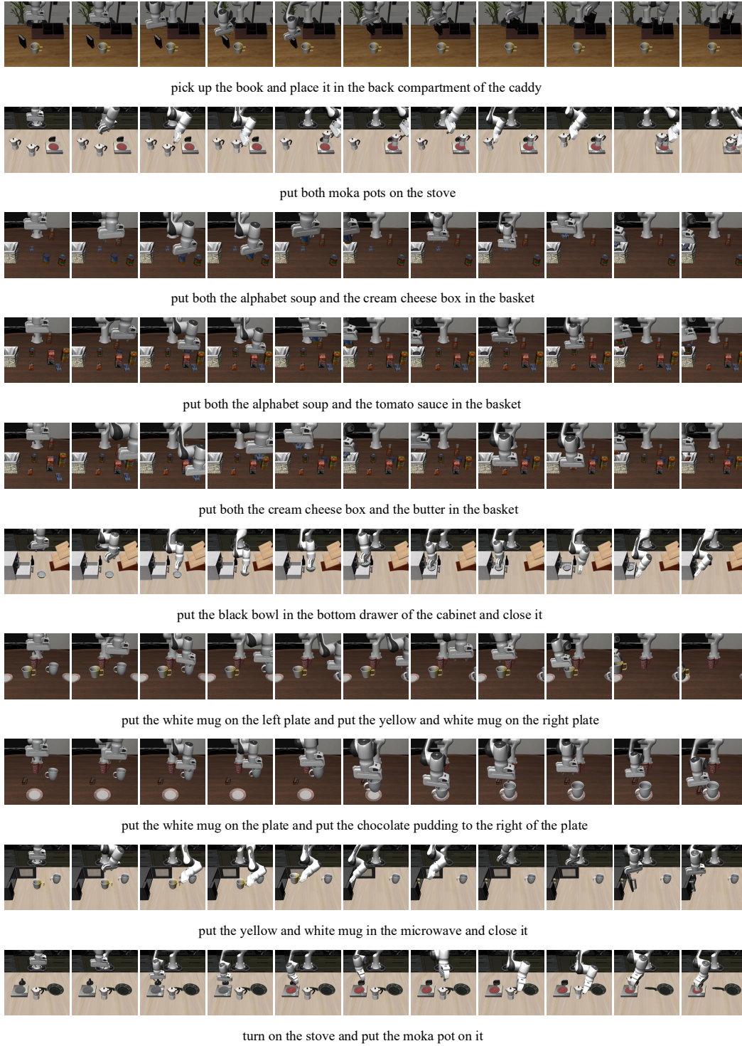
Figure 6: LIBERO-10 Visualization.
