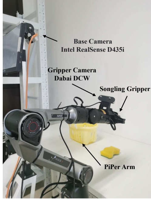
Figure 5: Real robot setup. The platform consists of a PiPer robotic arm with a Songling gripper, equipped with two complementary cameras: an Intel RealSense D435i base camera ( 1280 \times 720 ) and a Dabai DCW gripper-mounted depth camera ( 640 \times 480 ).
