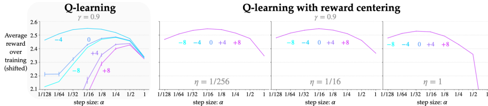
Figure 8: Parameter studies showing the sensitivity of the two algorithms’ performance on variants of the Access-Control Queuing domain. The error bars indicate one standard error, which at times is less than the width of the lines. Far left : Without centering, the performance of Q-learning differed significantly on the different variants over a broad range of the step-size parameter \alpha . Center to right : With centering, the performance was about the same across the problem variants, and was quite robust to the choice of its parameter \eta . All the curves correspond to \gamma = 0.9 ; the trends were consistent across other discount factors.
