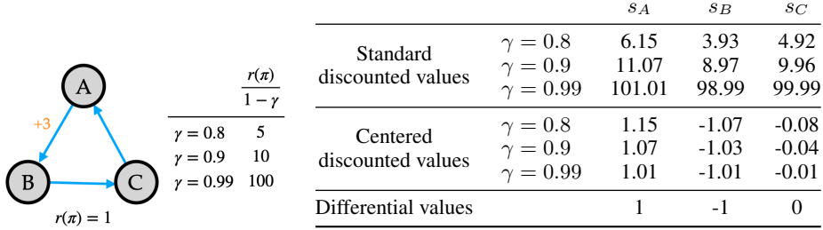
Figure 2: Comparison of the standard and the centered discounted values on a simple problem.
