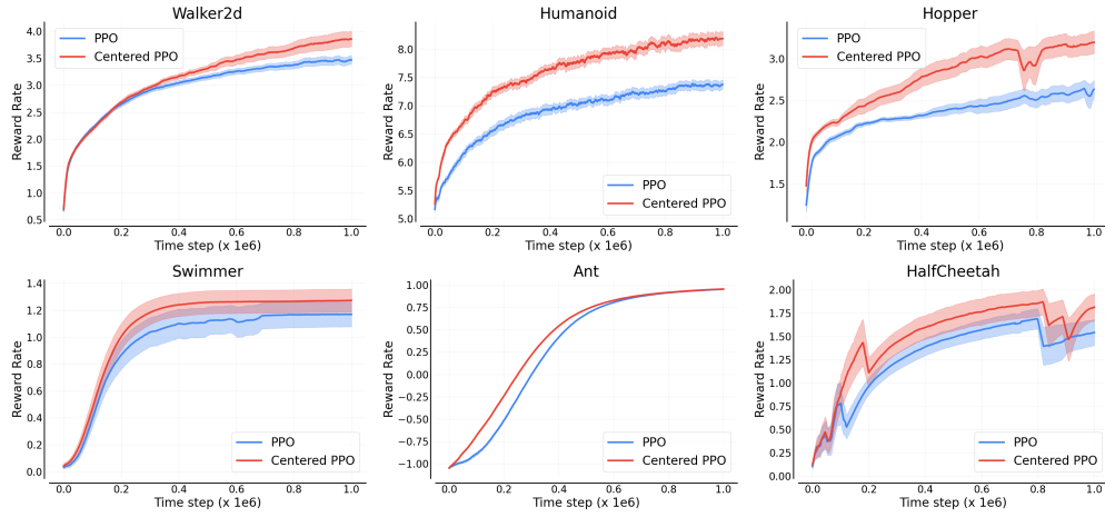
Figure 15: Learning curves for PPO with and without centering on continuing versions of six Mujoco domains. The solid lines and the shaded region denote the mean and one standard error over 10 independent runs.
