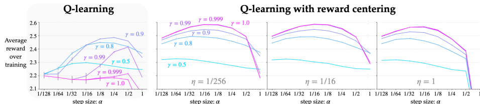
Figure 4: Parameter studies showing the sensitivity of the algorithms’ performance to their parameters on the Access-Control problem. The error bars indicate one standard error, which at times is less than the width of the lines.
