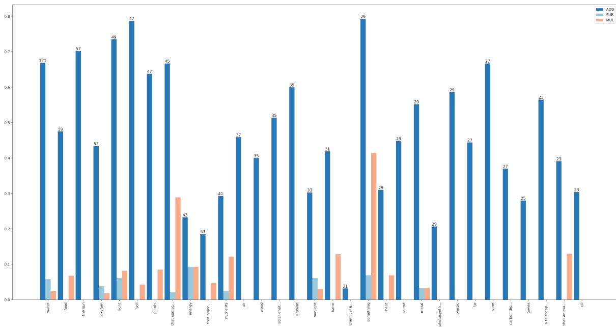
Figure 12: Object (ARG1).
