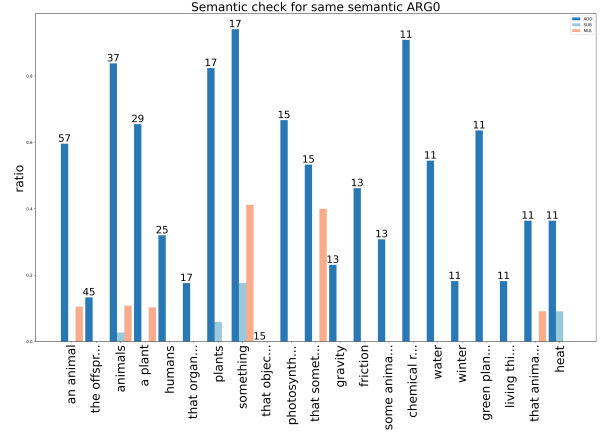
Figure 6: Arithmetic, s_1 \pm s_2 , for ARG0 with contents (dark blue: addition, shallow blue: subtraction, orange: element-wise production).
