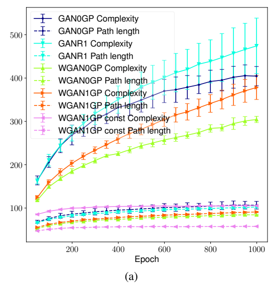
Figure 6: Experimental result for the computational complexity.
