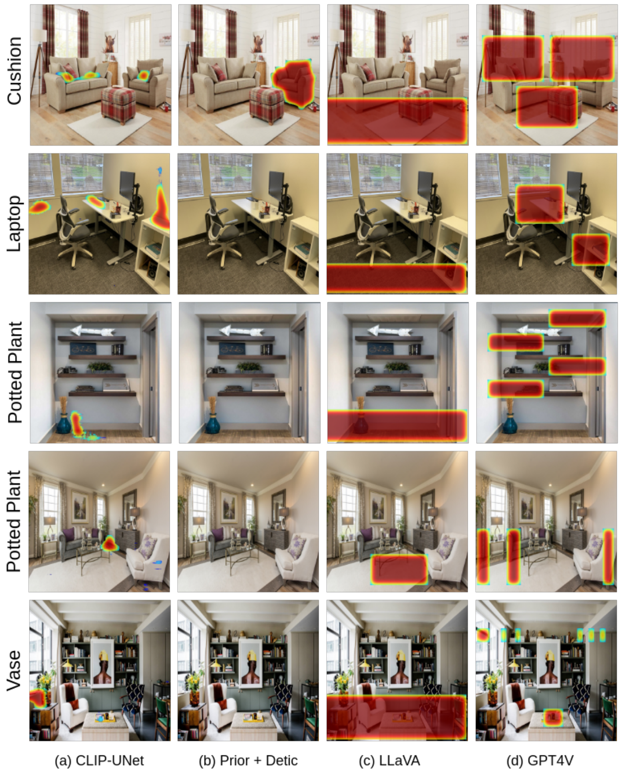
Fig. 11. Qualitative examples of SP masks predicted by all the baselines on SP Real val dataset
