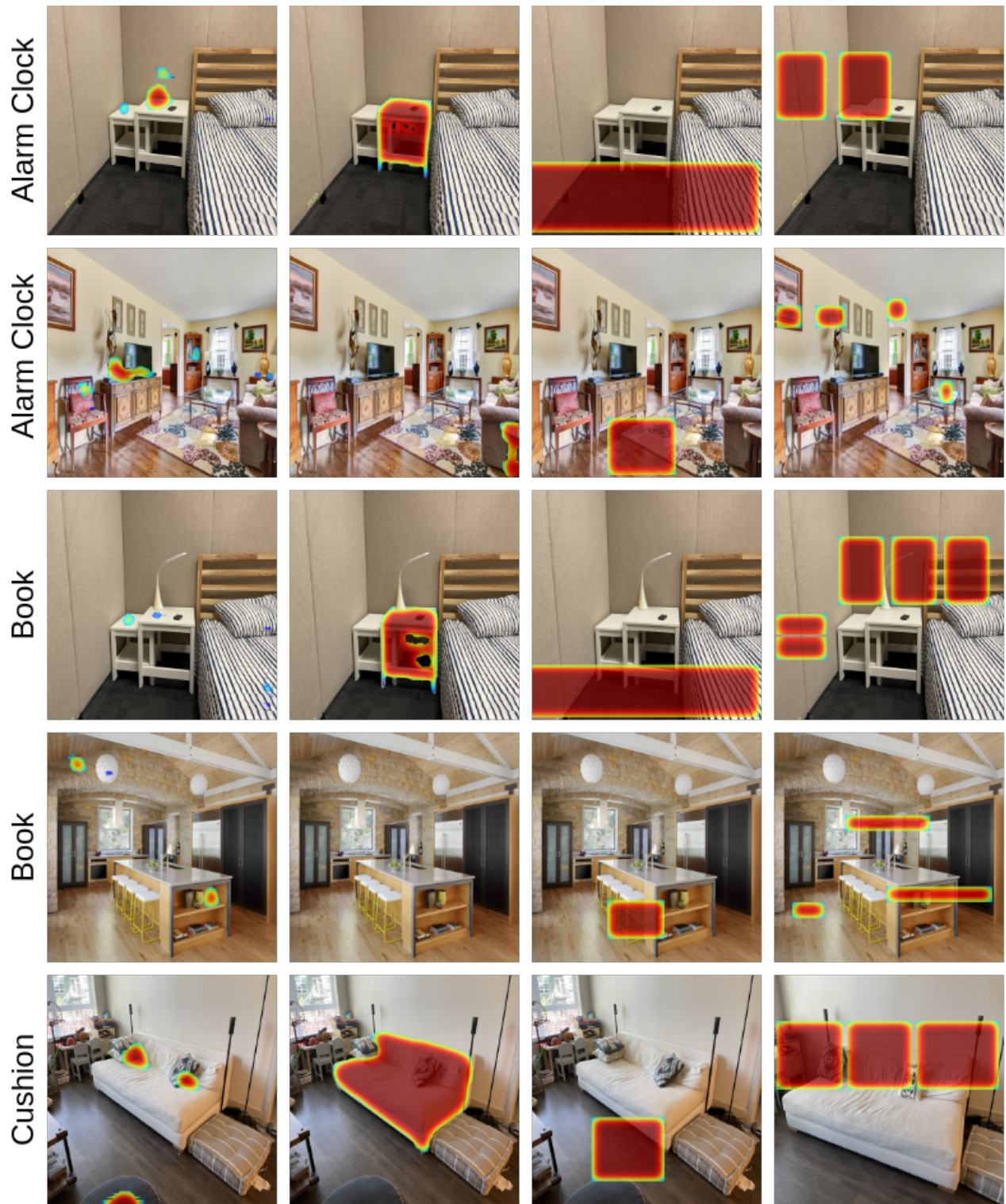
(a) CLIP-UNet
