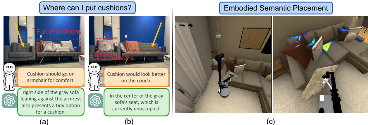
Fig. 1. Semantic Placement. Consider asking an agent to place cushions in a living room. In (a), the couch on the right is already full with cushions, and a natural human preference would be to place the cushion against the backrest of the armchair. In (b), a natural placement preference would be center of the couch. We propose the problem of Semantic Placement (SP) – given an image and a name of an object, a vision system must predict a semantic mask indicating a valid placement for the object in the image. For both (a) and (b) GPT4V gives meaningful natural language responses but, as we show, struggles to localize regions precisely in pixel space. (c) Our SP predictions enable a Stretch robot [1] from Hello Robot to perform Embodied Semantic Placement (eSP) task within a photorealistic simulated environment.
