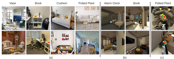
Fig. 3. Qualitative examples of SP masks predicted by our CLIP-UNet model pretrained on LAION-SP dataset and finetuned on HSSD images. (a) shows evaluation results on real image dataset from LAION [9], (b) shows results on images from HSSD dataset [13], and (c) shows results of placement predicted while evaluating tidying robot on Embodied Semantic Placement (eSP).
