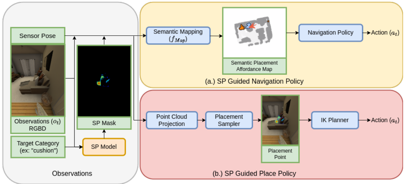
Fig. 7. Embodied Evaluation Pipeline. We build a two-stage modular policy consisting of: 1.) SP Guided Navigation Policy: Uses frontier exploration and semantic placement affordance 2D map to navigate to placement area, 2.) SP Guided Place Policy: Uses predicted SP mask, projects it onto a pointcloud to sample placement point and uses IK planner to place the object.
