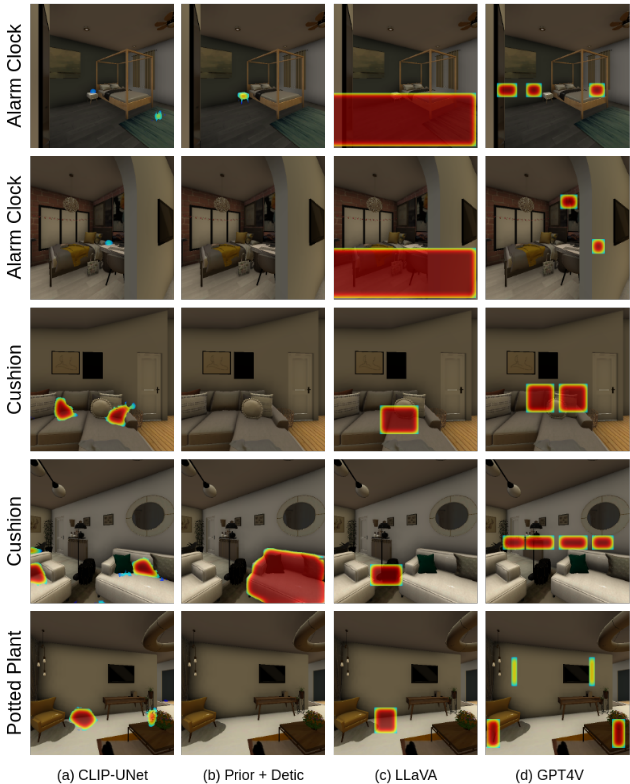
Fig. 12. Qualitative examples of SP masks predicted by all the baselines on SP HSSD val dataset
