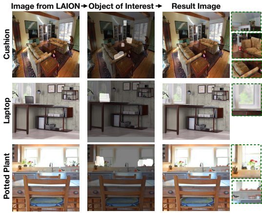
Fig. 4. Qualitative Examples of Generated Images. We present three examples of Cushion, Laptop, and Potted Plants, which include raw images queried from LAION (left), identified objects of interest and their segmentation masks obtained from SAM (middle), and the result images after Inpainting , Flitering , and Quality Enhancement steps (right). For clarity, we have magnified the inpainted regions, highlighted in green dotted boxes.
