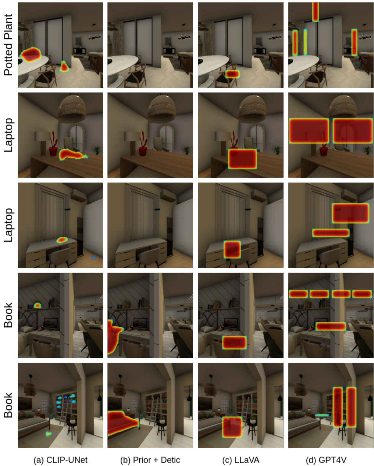
Fig. 13. Qualitative examples of SP masks predicted by all the baselines on SP HSSD val dataset
