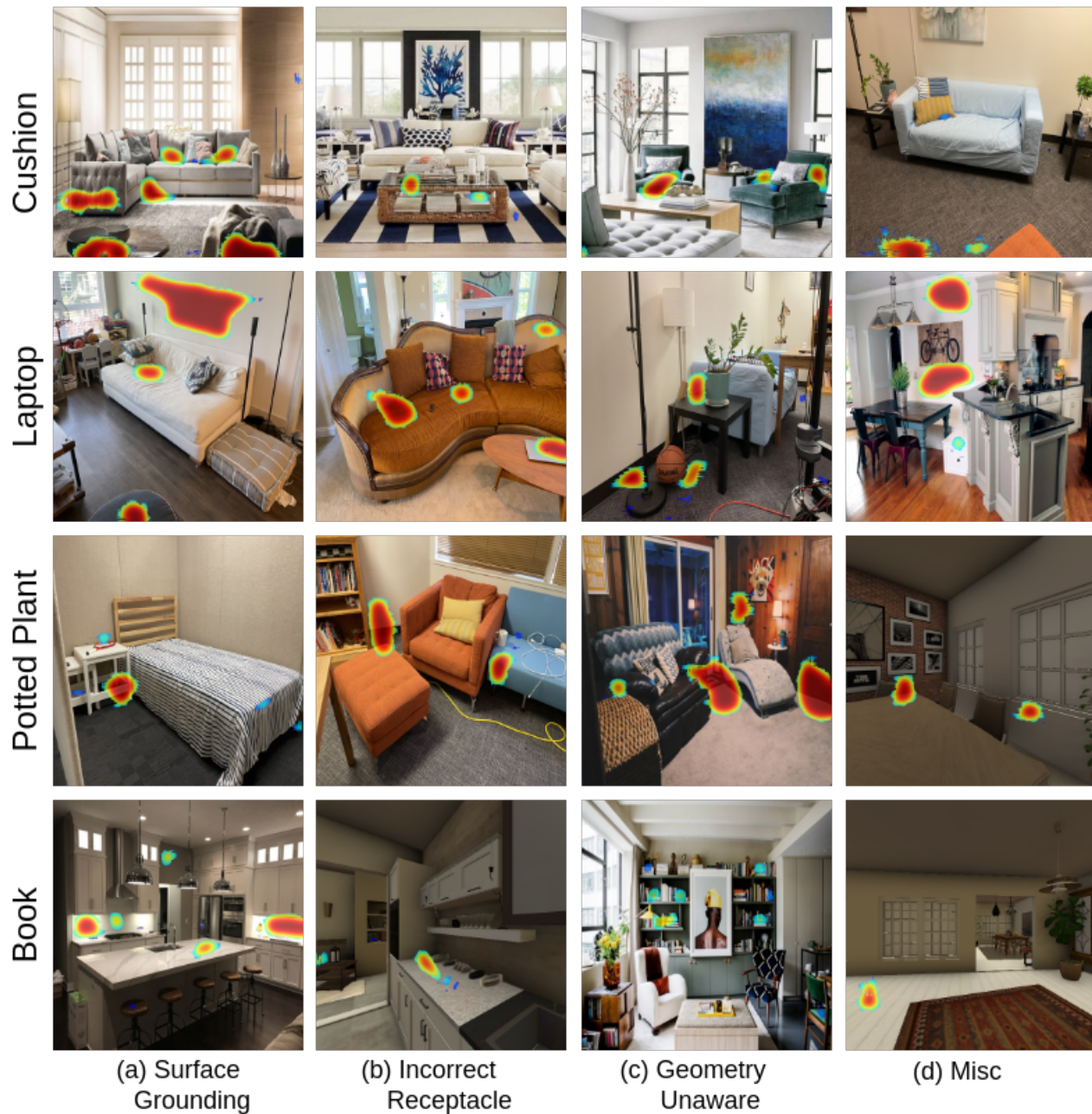
Fig. 14. Qualitative examples of failure modes of SP mask prediction by our approach
