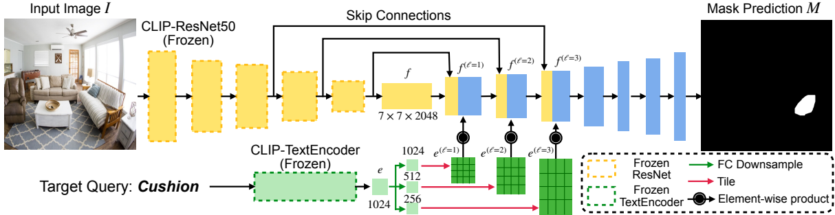
Fig. 5. CLIP-UNet for the SP task
