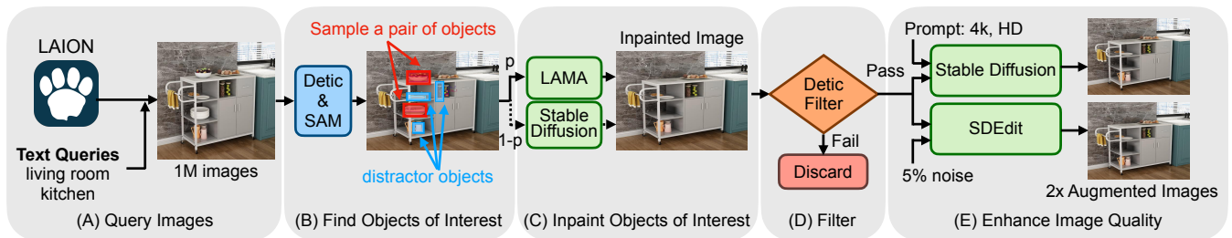
Fig. 2. Automatic Training Dataset Generation Pipeline Utilizing Foundation Models and Web Data. Our pipeline consists of five steps: (A) Query Images , (B) Find Objects of Interest , (C) Inpaint Objects of Interest , (D) Filter , (E) Enhance Image Quality
