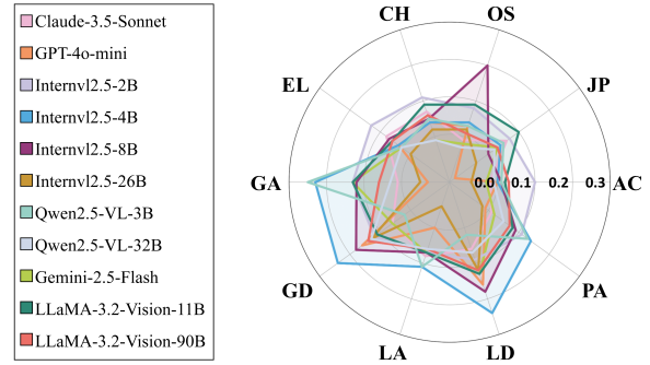
Figure 4: Trait-level score improvements after reflection via CAFES across different student MLLMs.
