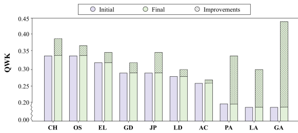
(a) Qwen2.5-VL-3B
