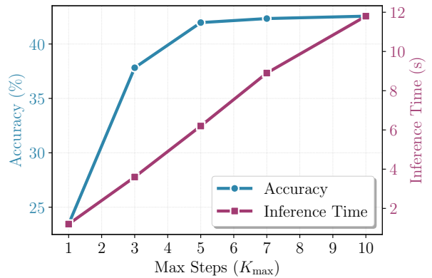
Figure 2: Impact of maximum reasoning steps on performance and efficiency. The figure shows accuracy and inference time as functions of maximum allowed reasoning steps.
