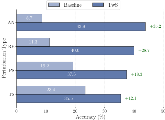
(b) Performance improvement
