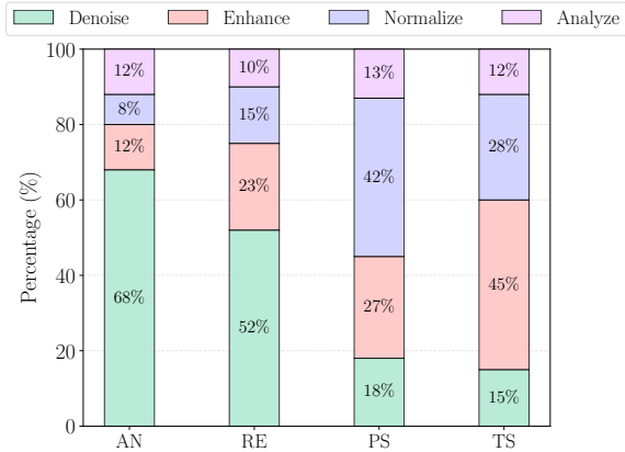
(a) Operator usage distribution
