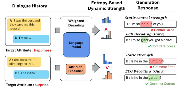
Figure 1: Controllable Dialog Generation method based on dynamic weighting with Eco Decoding. By dynamically determining the weights between the language model probability distribution and the attribute control probability distribution, it is possible to perform attribute control while maintaining fluency.
