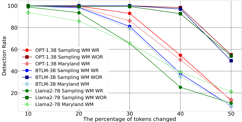
Figure 1: The impact of paraphrasing attacks on the detection rate of watermarked texts.
