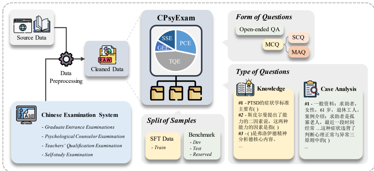
Figure 1: Overview of dataset constructing pipeline.
