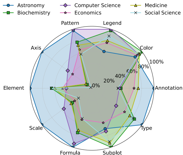
Figure 1: Radar plot of chart complexity across domains by comparing various visual design features, computed from 500 sampled charts per domain. Each axis represents a normalized design element contributing to overall chart complexity (formally defined later as the Chart Complexity Vector, or CCV). The domain-specific differences motivate our complexity-aware chart selection strategy.
