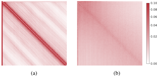
Figure 3: Attention maps of a single head from the first MHA module of BERT Base (a) and Base + Conv (b) (Section 3.5), averaged over 10^3 validation sequences to show the sequential locality preference of a typical attention head (see Appendix C for all heads). Each row corresponds to a query token position, each column to a key position. Adding the convolution module encourages attention layers to learn long-range content-based interactions over short-range position-based interactions.
