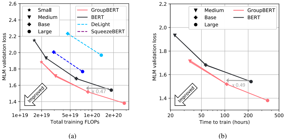
Figure 4: The GroupBERT model architecture is Pareto efficient on pre-training masked language modeling task. As well as comparing against the original BERT baseline, we tested transformers that use grouped transformations like SqueezeBERT and the uniform version of DeLight. For all models we tuned the learning rate to maximize their task performance. (a) Mean MLM validation loss \pm standard deviation plotted against the total pre-training FLOPs. (b) Mean MLM validation loss \pm standard deviation plotted against the total time for pre-training.
