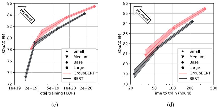
Figure 5: Median SQuAD F1 and Exact Match scores \pm standard deviation of the GroupBERT and BERT model families plotted against the total pre-training FLOPs (a,c) and against the total time to pre-train (b,d).
