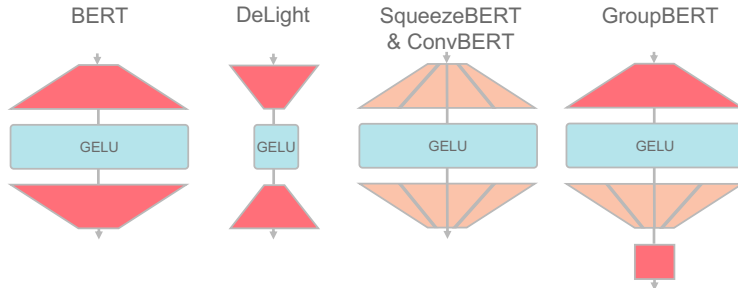
Figure 2: Schematic diagram showing the comparison of FFN implementations of different transformer variants that rely on grouped matrix multiplications.
