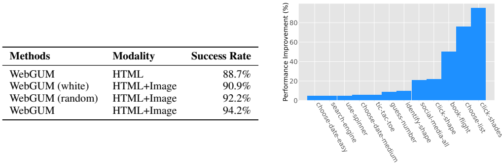
Figure 3: (Left) Average success rate with white/random image inputs. The results imply that WebGUM successfully leverages multimodal information from temporal and local perception tokens. (Right) Top-10 performance improvement among MiniWoB++ by adding image modality to HTML. We subtract the success rates to compute absolute improvement: (SR \text{ of WebGUM (HTML+Image)}) - (SR \text{ of WebGUM (HTML)}) . Image modality is leveraged for multi-step tasks with dynamic page transitions or tasks that require visual concept understanding (e.g. book-flight or click-shape ). See Appendix G and L for the details.
