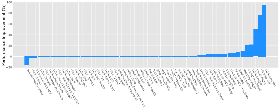
Figure 7: Performance improvement by adding image modality to HTML on 56 tasks from MiniWoB++. We subtract the success rates: (\text{Success Rate of WebGUM(HTML+Image)}) - (\text{Success Rate of WebGUM(HTML)}) .
