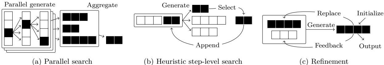
Figure 4: Three meta-generation patterns.
