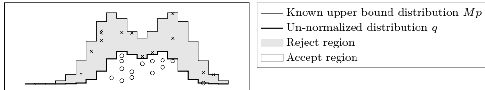
Figure 5: In rejection sampling, the aim is to sample from a distribution q whose normalizing constant is unknown. To do so, use a known distribution p that serves as an upper bound for the unknown distribution when scaled by a constant, i.e., for some constant M and all values y , Mp(y) \geq q(y) . Next, obtain a sample y \sim p and accept this sample with probability q(y)/Mp(y) , otherwise reject the sample and repeat the process. This is equivalent to sampling from q .
