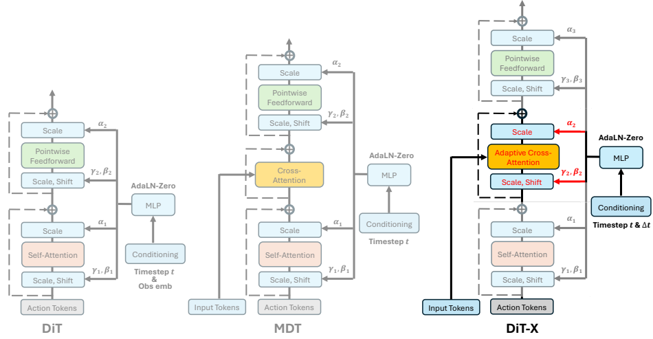
Figure 5: DiT-X Block. Unlike DiT (self-attention only) and MDT (basic cross-attention), DiT-X applies AdaLN-Zero conditioning to low-dimensional robot state inputs, and adjusts cross-attention input and output with learned scaling and shift parameters, ensuring adaptive and fine-grained feature interactions between action tokens and multi-modal input tokens. This design enables efficient handling of both low-dimensional control signals and high-dimensional perceptual inputs.
