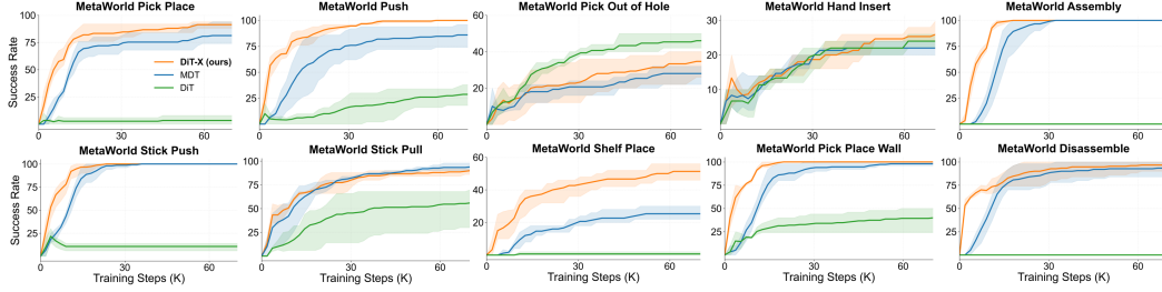
Figure 14: Comparison between DiT, MDT, and ManiFlow’s DiT-X block: Language-conditioned multi-task learning curves for 10 MetaWorld hard tasks. DiT-X demonstrates faster convergence towards higher accuracy, highlighting superior multi-modal conditioning capabilities.
