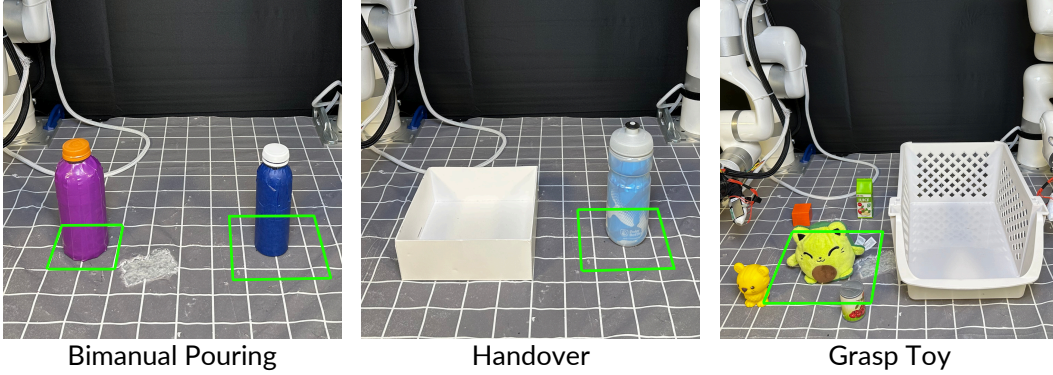
Figure 19: Testing area of Bimanual Tasks. The testing areas for our bimanual tasks are highlighted as green quadrilaterals. (i) Bimanual Pouring designates a 10.5\text{cm} \times 10.5\text{cm} area for the target bottle and a 15\text{cm} \times 15\text{cm} area for the pouring bottle. (ii) Handover positions the bottle within a 15\text{cm} \times 15\text{cm} area, while the box may experience displacement perturbations of approximately 1.5\text{cm} in all directions. (iii) Toy Grasping places the toy within a 21\text{cm} \times 21\text{cm} area, with distractors randomly arranged around it. Additionally, the basket may undergo front-back displacement perturbations of around 2.5\text{cm} in each direction.
