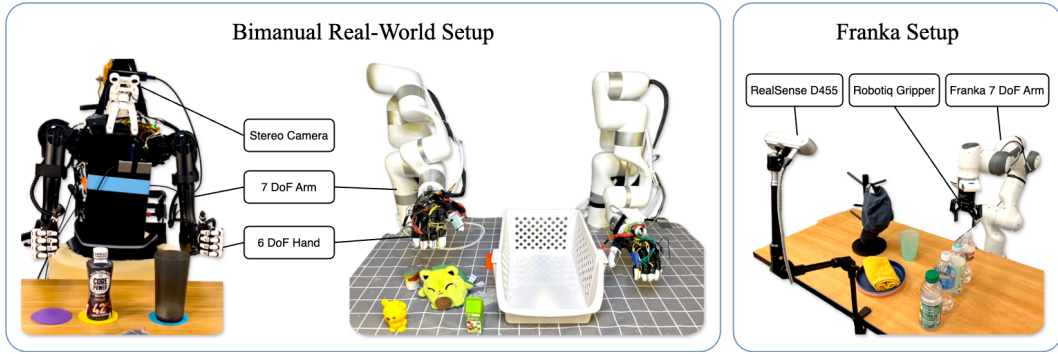
Figure 17: Real-World Setup. The experimental setup includes three configurations: (1) a bimanual Unitree H1 humanoid robot with 7-DoF arms, anthropomorphic hands, and a gimbal-mounted stereo camera; (2) a Bimanual 7DoF xArm setup with PSYONIC Ability Hands and an Intel RealSense L515 camera; and (3) a Franka Emika Panda robot with a Robotiq gripper and a statically positioned Intel RealSense D455 camera.
