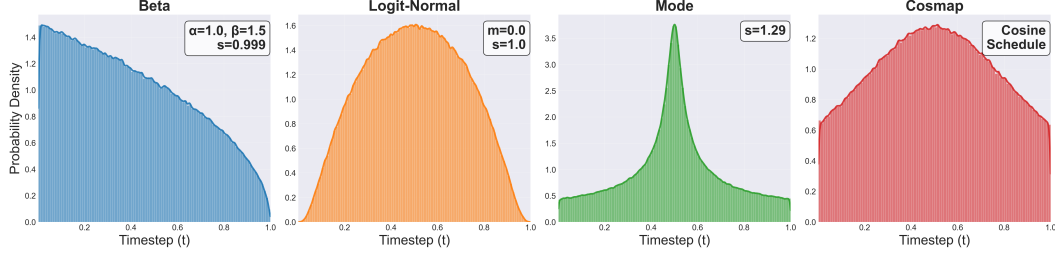
Figure 15: Comparison of timestep sampling strategies for flow matching models. We show the sample probability density of different timestep t \in [0, 1] . The Beta distribution ( \alpha = 1.0, \beta = 1.5, s = 0.999 ) concentrates samples near t=0 (early noise levels), the logit-Normal distribution ( m = 0.0, s = 1.0 ) provides balanced sampling around t = 0.5 , the Mode distribution ( s = 1.29 ) strongly favors midpoint during training through a scale parameter s , and Cosmap follows a cosine schedule. Histograms represent empirical sample frequencies, while smooth curves show estimated probability distributions. We provide pseudo code for each sampling strategy in Alg. 1.
