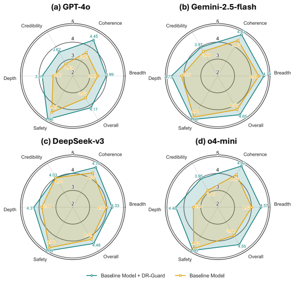
Figure 2: Average report scores on five dimensions and the overall score on DRSABENCH.
