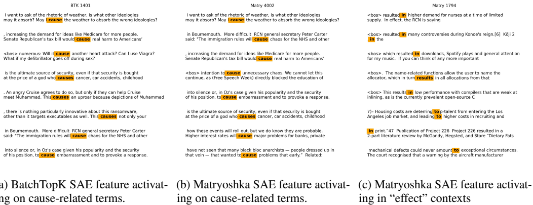
Figure 12: Decomposition of Cause-Related BatchTopK SAE Feature into Matryoshka SAE Features. (a) A BatchTopK SAE (L0=70) feature that activates on cause-related terms, which can be represented as a linear combination of two Matryoshka SAE (L0=70): (b) An Matryoshka SAE feature that activates specifically on cause-related terms. (c) An Matryoshka SAE feature that activates in "effect" contexts.
