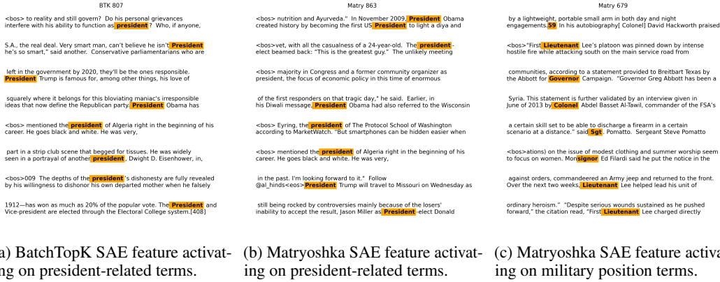
Figure 11: Decomposition of President-Related BatchTopK SAE Feature into Matryoshka SAE Features. (a) A BatchTopK SAE (L0=70) feature that activates on president-related terms, which can be represented as a linear combination of two Matryoshka SAE (L0=70): (b) A Matryoshka SAE feature that activates specifically on president-related terms. (c) A Matryoshka SAE feature that activates on military position terms.
