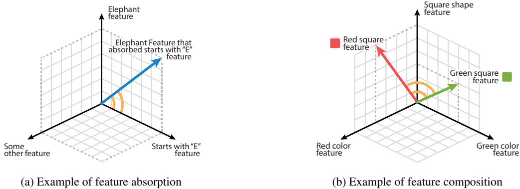
Figure 2: Illustration of feature absorption and feature composition: (a) In feature absorption, specific features like “elephant” absorb broader features like “starts with E”. (b) In feature composition, independent concepts like “red color” and “square form” are merged into composite features.
