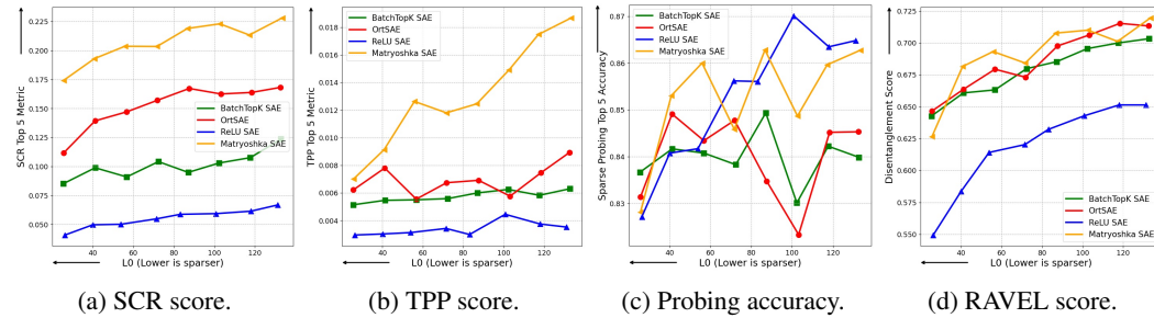
Figure 6: Results on SAE Bench. (a) Spurious Correlation Removal: OrtSAE outperforms traditional SAEs but achieves lower scores than Matryoshka. (b) Targeted Probe Perturbation: OrtSAE shows modest improvements over traditional SAEs, while Matryoshka demonstrates the strongest performance. (c) Sparse Probing: OrtSAE maintains accuracy comparable to baseline methods. (d) RAVEL: OrtSAE achieves scores similar to both BatchTopK and Matryoshka SAEs.
