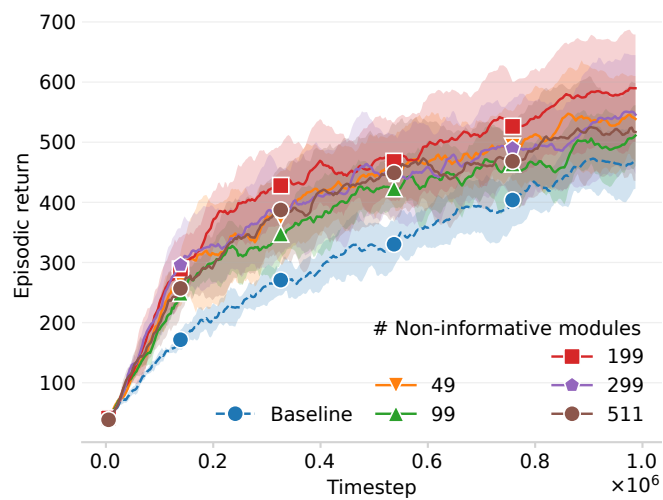
Figure H.1: Scalability of the attention heads to retrieve useful information from previous modules in extremely long task sequences. The figure compares the episodic return curve of the baseline method (trained from scratch) to CompoNet with an increasing number of non-informative previous modules and a single module that is trained to solve the current task. Specifically, the task at hand is the sixth task of the SpaceInvaders sequence. Lines and contours respectively represent the mean and standard deviation of 5 runs with different random seeds. Note that the total number of previous modules for each curve is the number of non-informative modules, shown in the legend, plus one, corresponding to the informative (i.e., trained) module.
