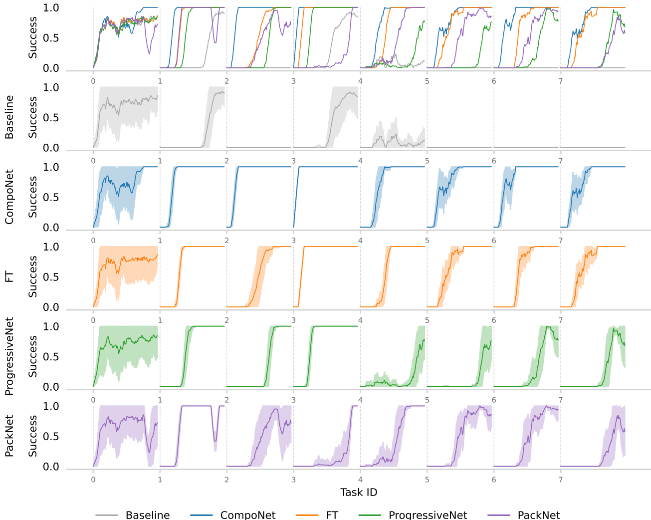
Figure F.3: Success curves of the different methods in the Freeway sequence. Results from 10 seeds are aggregated.
