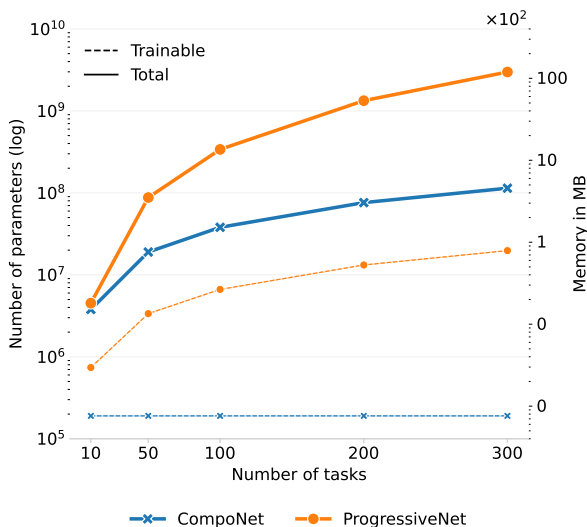
Figure B.1: Growth in memory of CompoNet and ProgressiveNet models as the number of tasks (assuming an NN module per task) increases. The count is given in the total number of parameters, depicted with solid lines, and in the number of trainable parameters (not frozen), in dashed lines. Note that we assume 32-bit floats are used to represent the parameters of the models. Hyperparameters correspond to the ones utilized in the Meta-World sequence: d_{\text{enc}} = 39 , d_{\text{model}} = 256 , and |\mathcal{A}| = 4 .
