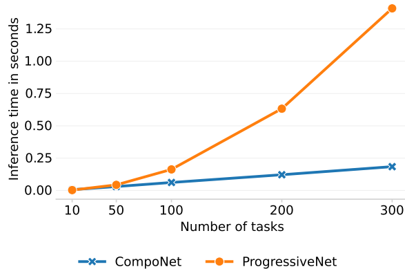
Figure C.1: Empirical computational cost of inference of CompoNet and ProgressiveNet with respect to the number of tasks (assuming one module is instantiated for every task). Results depict the average inference time over one minute of recording. This ensures a minimum of 40 inferences to compute the estimate ( 40 = 60/1.5 ). Hyperparameters are: d_{\text{enc}} = 39 , d_{\text{model}} = 256 , and |\mathcal{A}| = 4 . Results were measured in a machine with an AMD EPIC 7252 CPU and an NVIDIA A5000 GPU.
