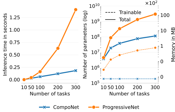
Figure 3: Empirical computational cost of inference (left) and growth in the number of parameters (right) with respect to the number of tasks for CompoNet and ProgressiveNet methods. Hyperparameters are: d_{\text{enc}} = 64 , |\mathcal{A}| = 6 , d_{\text{model}} = 256 , and a batch size of 8. Measurements have been taken in a machine with an AMD EPYC 7252 CPU and an NVIDIA A5000 GPU.
