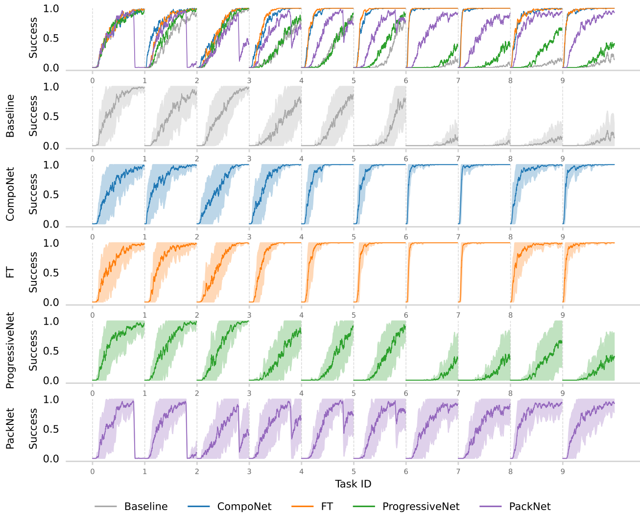
Figure F.2: Success curves of the different methods in the SpaceInvaders sequence. Results from 10 seeds are aggregated.
