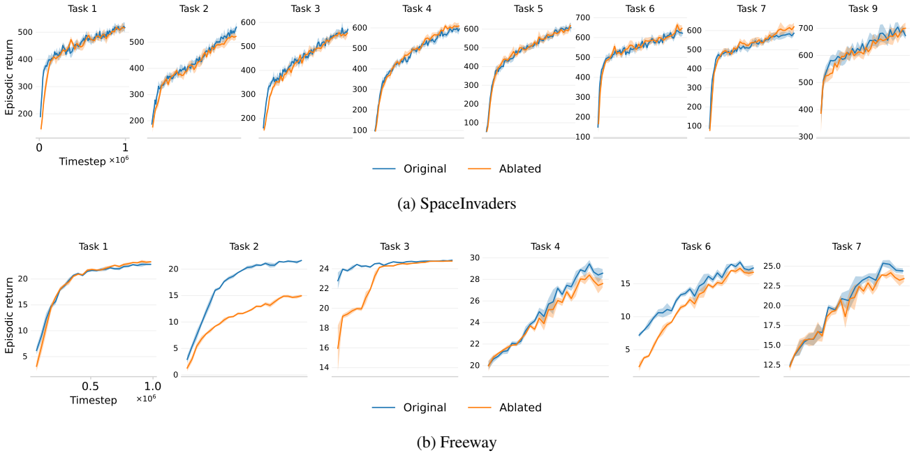
Figure G.1: Episodic return curves for the SpaceInvaders and Freeway sequences. Blue lines correspond to the original CompoNet architecture presented in Section 4, while orange lines represent the same architecture with no output attention head (referred to as Ablated ). Each curve is computed from the average result of 5 seeds and contours indicate standard error.
