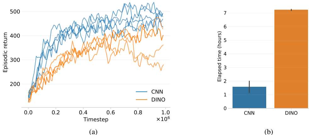
Figure A.1: Comparison of training an agent in the first task of the SpaceInvaders sequence using the representations generated by a pre-trained DINO model, and a CNN encoder that is trained with the agent. The leftmost figure compares both approaches in terms of episodic return, while the rightmost compares the total execution times to reach 1M timesteps. Both figures contain the results from 5 runs per setting.
