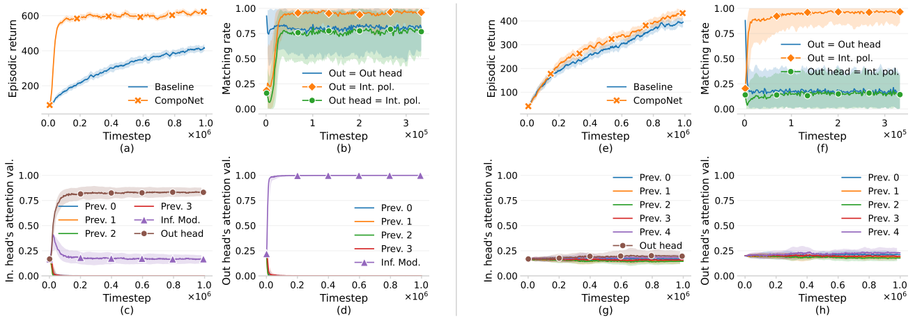
Figure 4: Empirical results on the fulfillment of objectives (i) and (iii) from Section 4 that motivated the design of CompoNet. In the leftmost figures, CompoNet is trained on the fifth task of SpaceInvaders with four non-informative previous policies that sample their output from a uniform Dirichlet distribution, and one policy trained to solve the current task ( Inf. Mod. ). In the rightmost figures, CompoNet is trained on the sixth task of SpaceInvaders with five non-informative previous policies. Results aggregate 10 random seeds. The matching rate indicates the frequency with which the action of the highest probability from the output of the last module, or some of its components, matches with each other. For clarity, the X axis of Figures 4.b and 4.f are shortened to the first 3 \times 10^5 timesteps.
