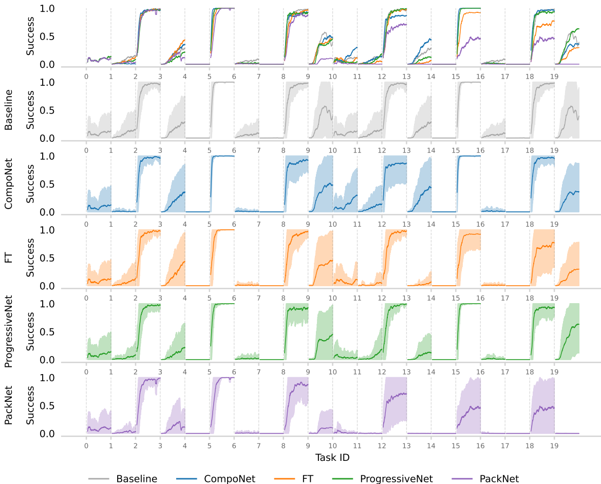
Figure F.1: Success curves of all methods in the Meta-World sequence. Results from 10 seeds are aggregated.
