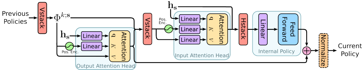
Figure 2: Diagram of the self-composing policy module. Vstack and Hstack successively represent row-wise and column-wise concatenation operations, while the normalization operation has been delimited with a dashed line to denote that it is optional and dependent on the nature of the action space. Finally, note that the only blocks with learnable parameters are the feed-forward block and the linear transformations.
