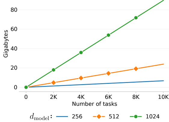
Figure B.2: Memory size in Gigabytes required by CompoNet with respect to the number of tasks for different d_{\text{model}} values. Hyperparameters correspond to the ones from the Meta-World sequence: d_{\text{enc}} = 39 , and |\mathcal{A}| = 4 .
