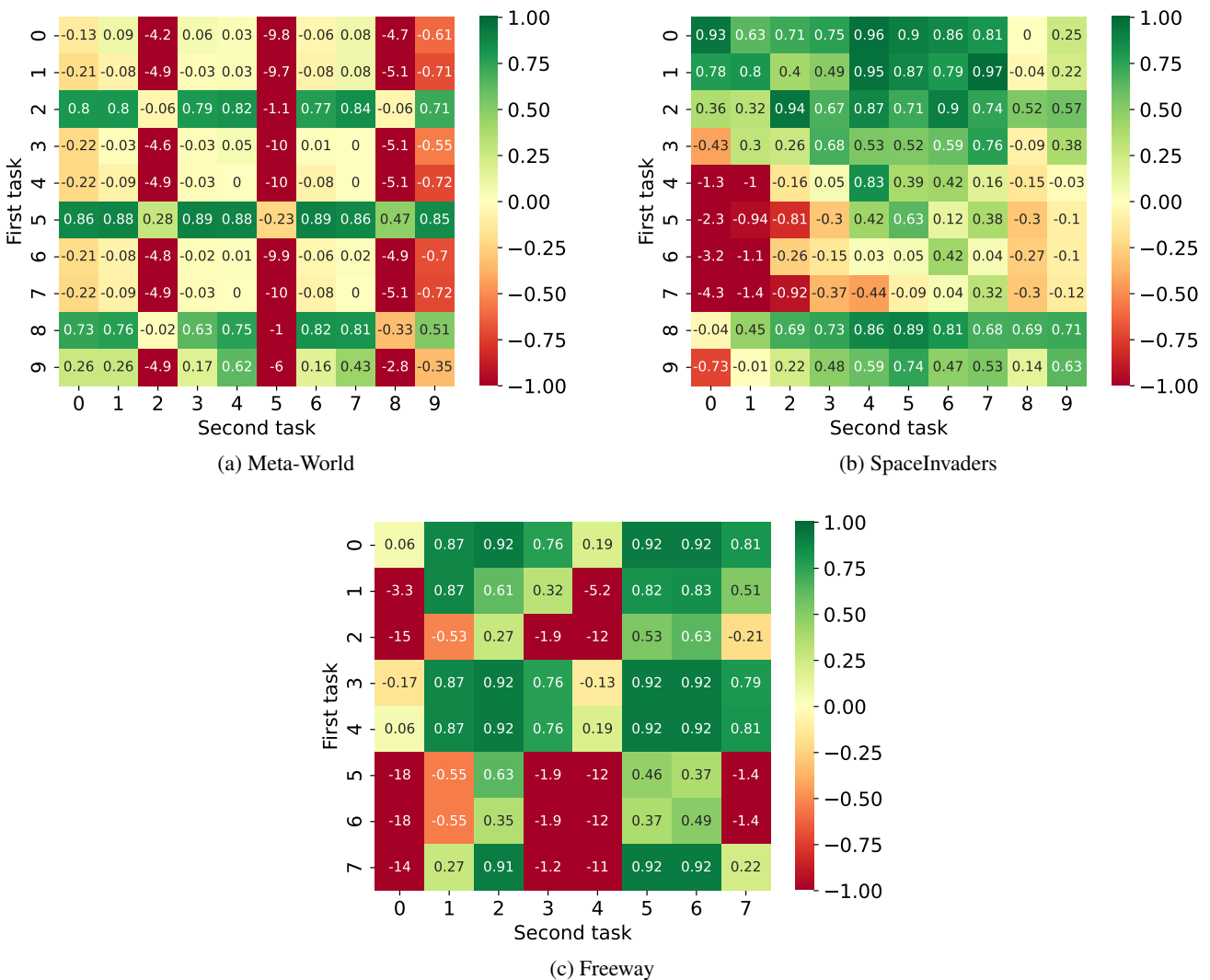
Figure D.2: Forward transfer matrices for all sequences. Each element in the matrices is computed as the average forward transfer of training a model from scratch in the first task (Y-axis) and fine-tuning it in the second (X-axis). Results aggregate values from 3 different random seeds. Note that Figure D.2a is a 10 \times 10 matrix and not 20 \times 20 , corresponding with the 10 different tasks that comprise the sequence, as the remaining 10 are repetitions of these.
