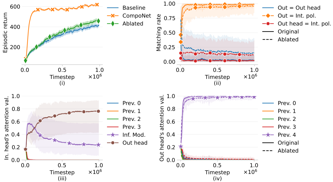
Figure G.2: Comparison of the original CompoNet design, an ablated version of CompoNet without the input attention head, and the baseline. The methods have been trained to solve the fifth task of the SpaceInvaders sequence using the hyperparameters from Appendix E, where the results of 10 seeds have been aggregated. In the case of the CompoNet models, five previous modules have been provided: four non-informative, and one trained to solve the current task (called Inf. Mod. and marked with stars). However, the output vectors of these modules have been shifted one element to the left, making the direct usage of Inf. Mod. an unviable approach although still maintaining useful information to solve the current task. In (i) the performance of the methods is compared in terms of episodic return; (ii) depicts the rate in which the outputs of different parts of the models match; finally, (iii) and (iv) respectively illustrate the evolution of the attention values for the input and output heads of the module being trained. Results show that the original version of CompoNet successfully employs the input attention head to extract information for the internal policy to solve the task at hand, greatly outperforming the ablated version and the agent trained from scratch.
