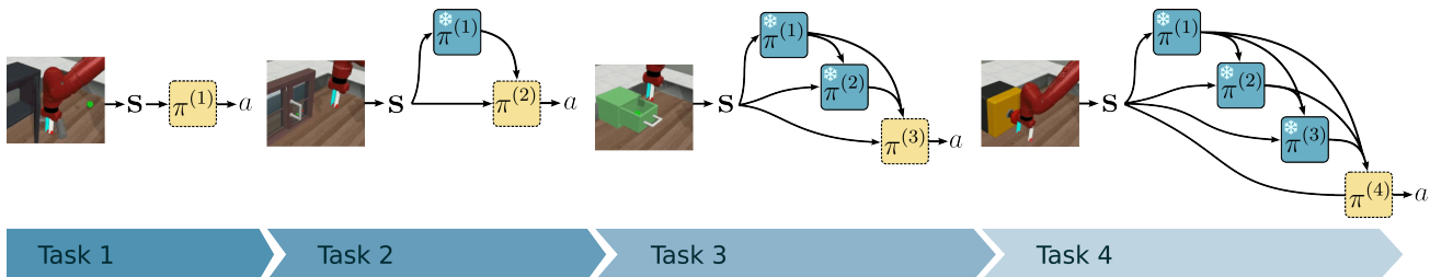
Figure 1: Evolution of the Self- Composing Policies Network architecture (CompoNet) across multiple tasks. Trainable self-composing policy modules are represented by light yellow blocks, and frozen modules are denoted by dark blue blocks. The initial task involves training a single policy module from scratch. Following the completion of each task, the trained module is frozen, and a new trainable module is introduced for the subsequent task. This process is repeated in every transition from one task to another. Importantly, each module, after the initial one, benefits from access to the current state of the environment alongside the outputs generated by the preceding policy modules.
